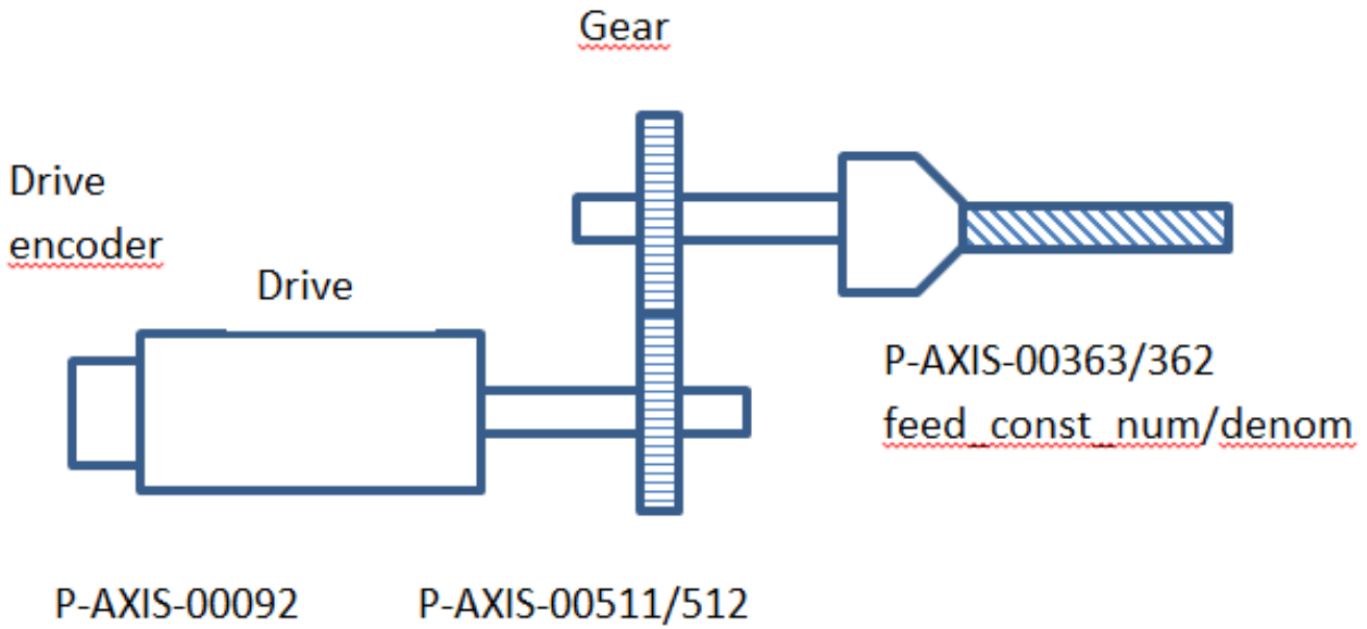
Fig. 51: Position scaling with fitted encoder
