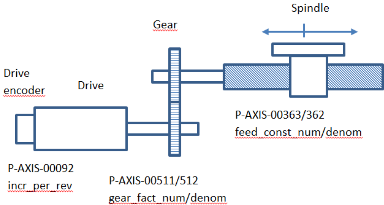
Fig. 49: Position scaling with rotary encoder
