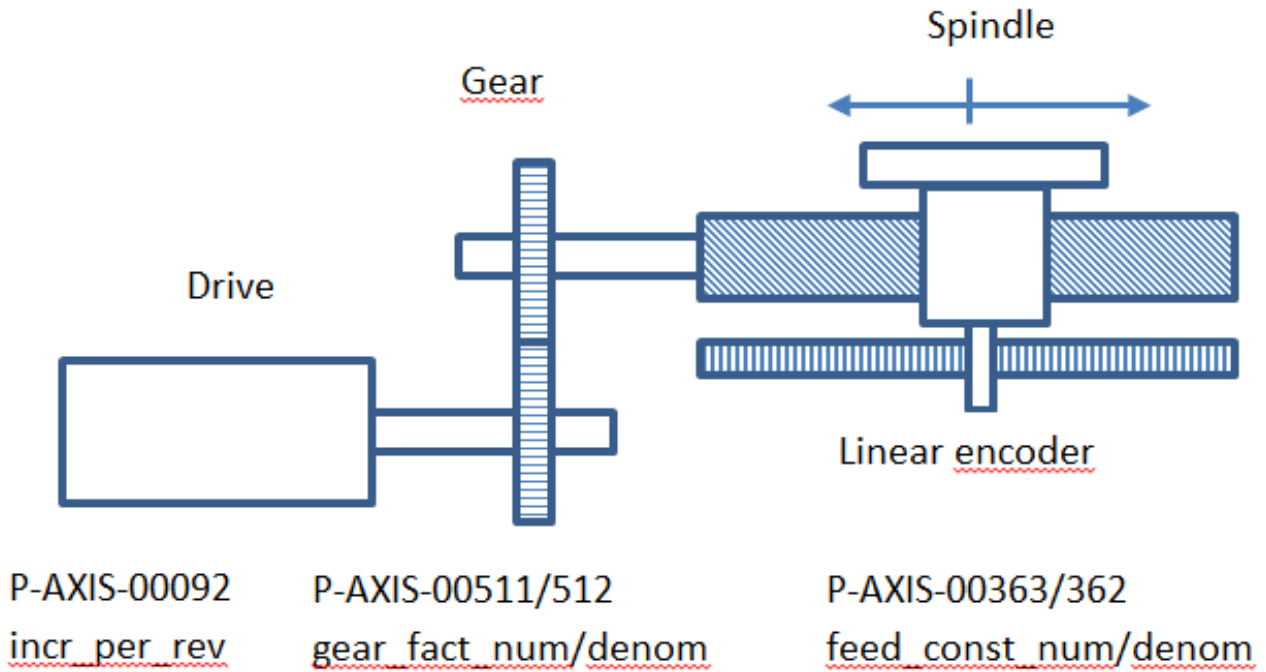
Fig. 50: Position scaling with linear encoder
