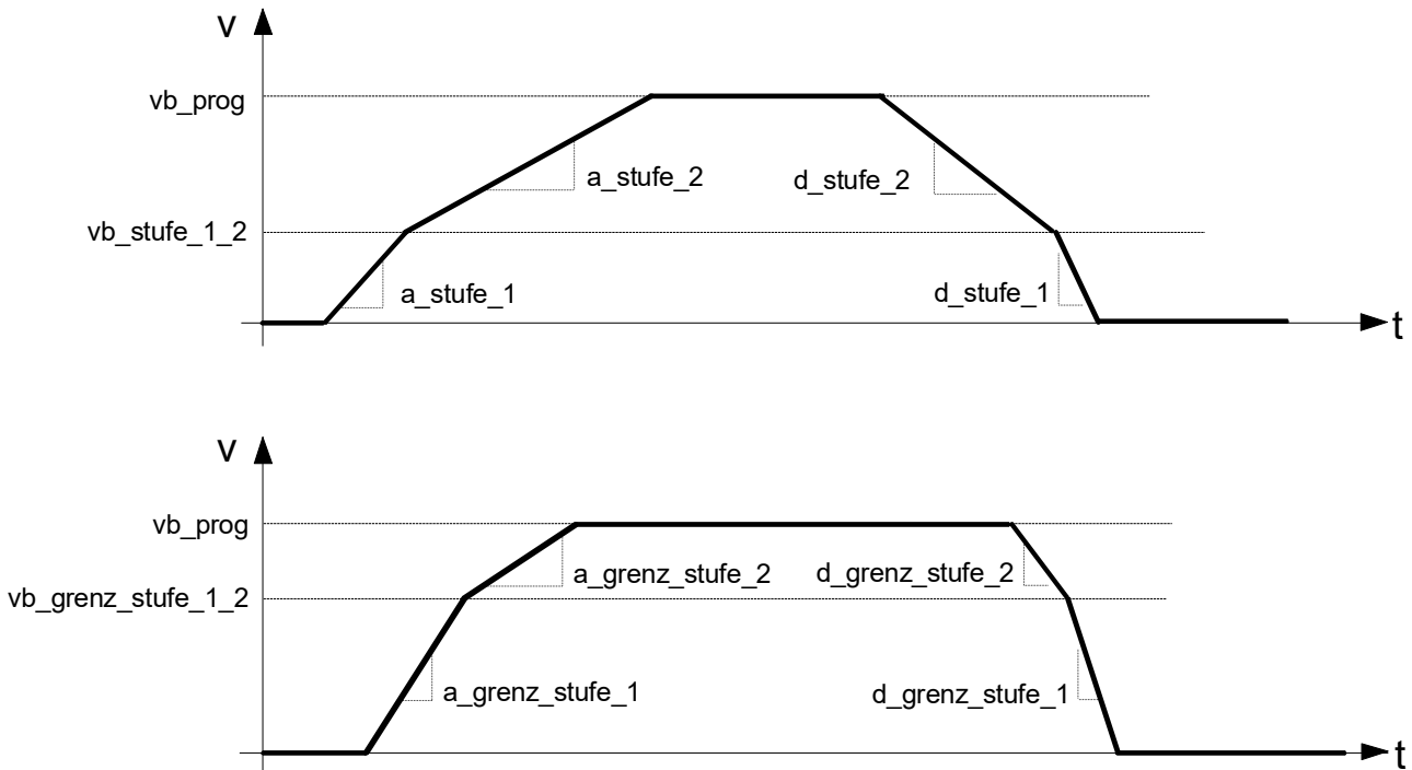
Fig. 17: Acceleration and deceleration parameters of the linear velocity profile
