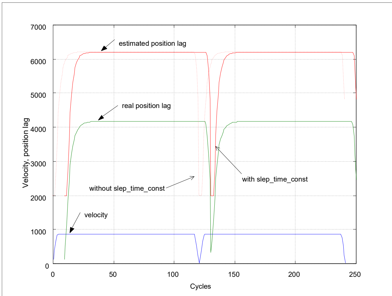
Fig. 28: Time constant to shift monitoring curve
