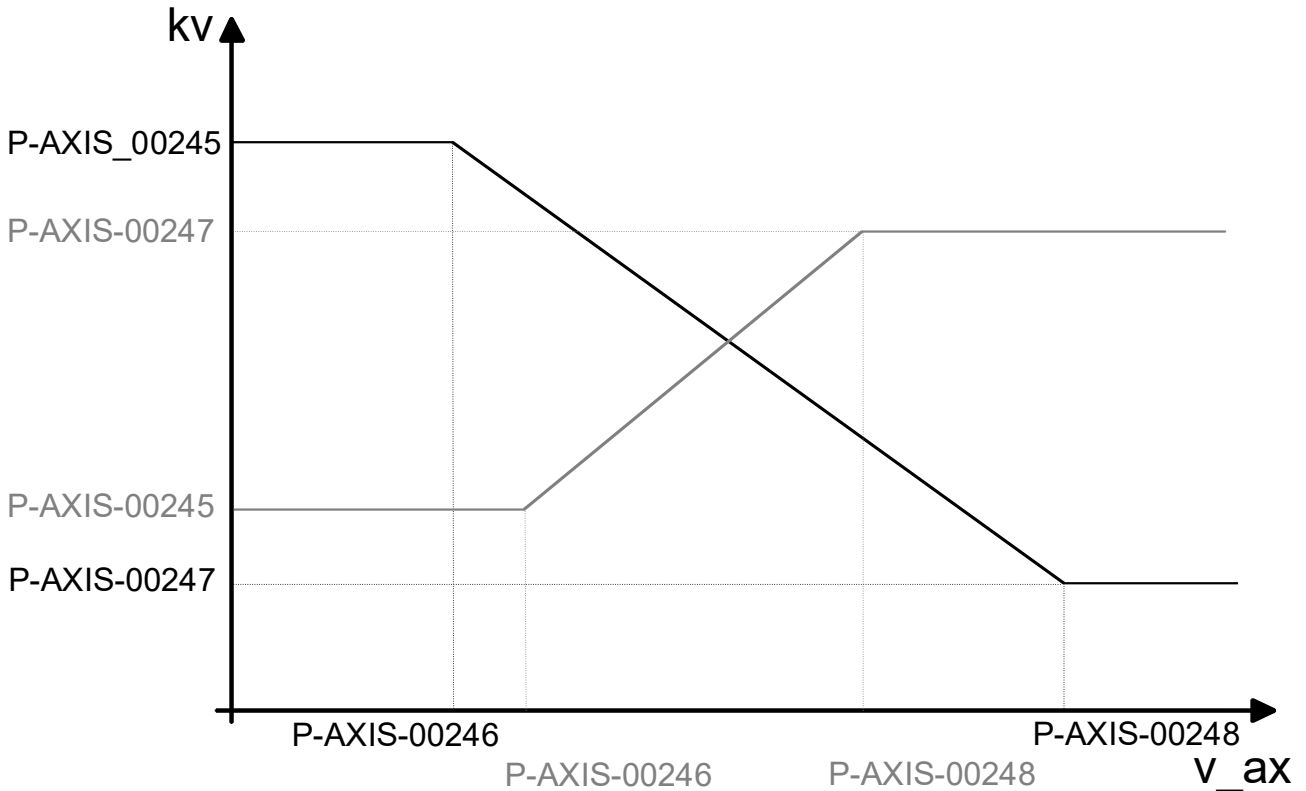
Fig. 29: Parameters of dynamic kv adjustment
