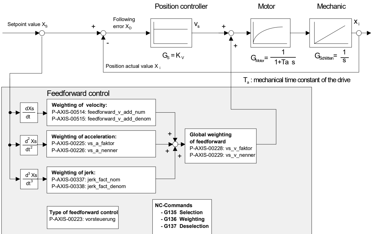
Fig. 31: Block diagram of feedforward control
