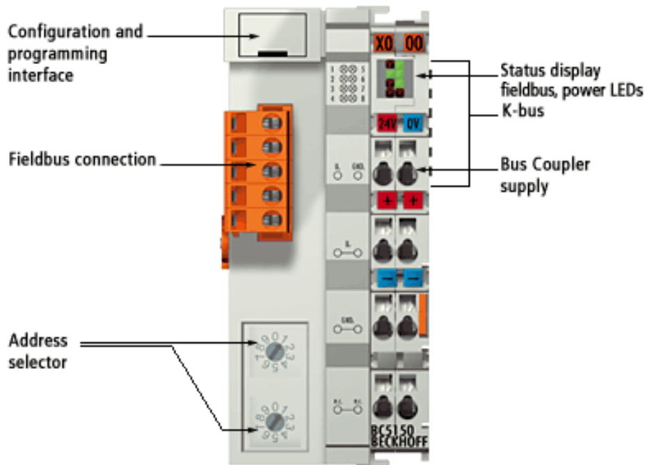
Fig. 1: BC5150 - Bus Terminal Controller for CANopen
