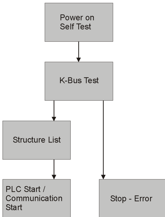
Fig. 21: Start-up behavior of the Bus Terminal Controller
