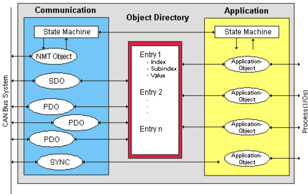
Fig. 74: CANopen Device Model
