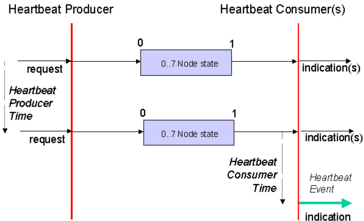
Fig. 77: Schematic diagram: "Heartbeat procedure"
