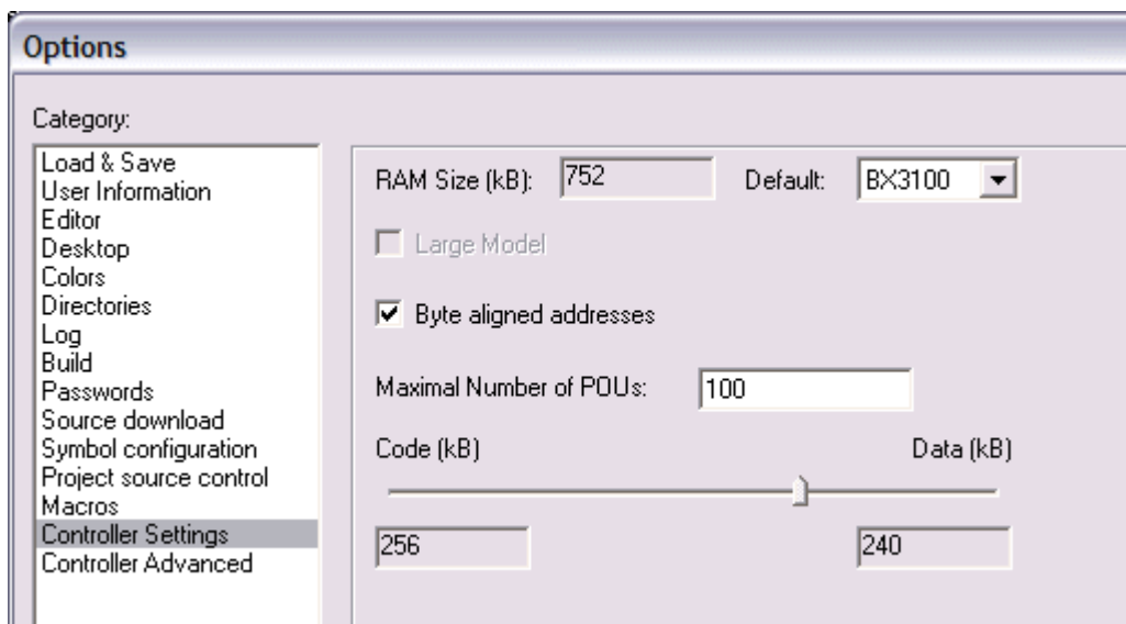
Fig. 50: Controller settings
