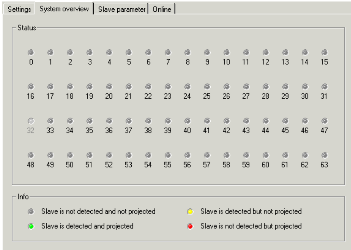
Fig. 24: KS2000 - AS-i system overview
