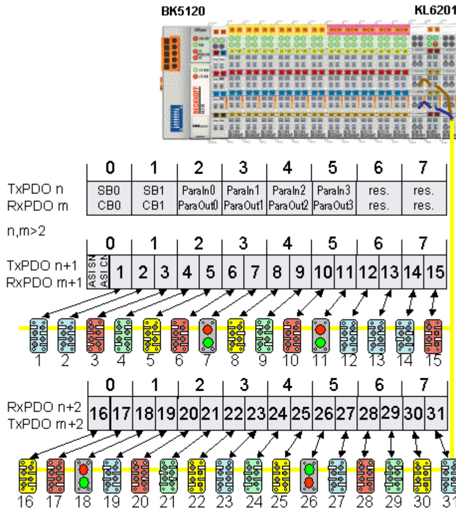
Fig. 34: Mapping of the AS-i data to the CANopen process data objects for the 22-byte process image
