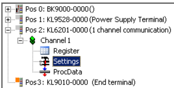
Fig. 20: KS2000 branches for channel 1 of the KL6201
