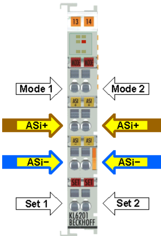
Fig. 16: Connection of the AS interface
