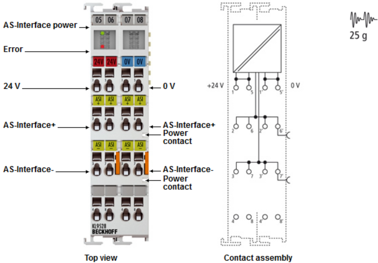
Fig. 4: KL9528 - AS-i Power Supply Terminal
