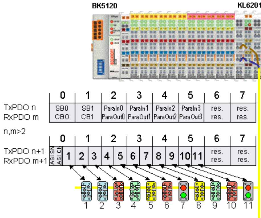
Fig. 33: Mapping of the AS-i data to the CANopen process data objects for the 12-byte process image
