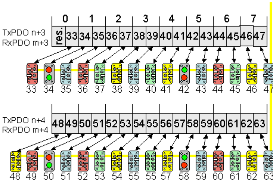
Fig. 35: Mapping of the AS-i data to the CANopen process data objects for the 38-byte process image
