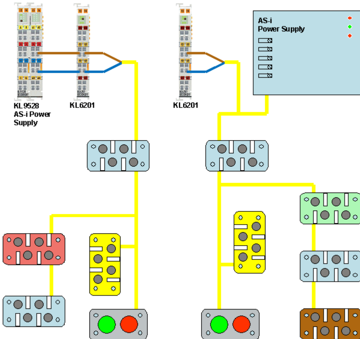
Fig. 17: Wiring of the AS interface
