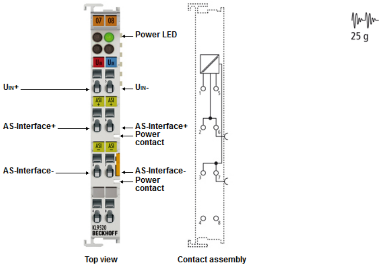
Fig. 5: KL9520 - AS-i potential feed terminal with filter
