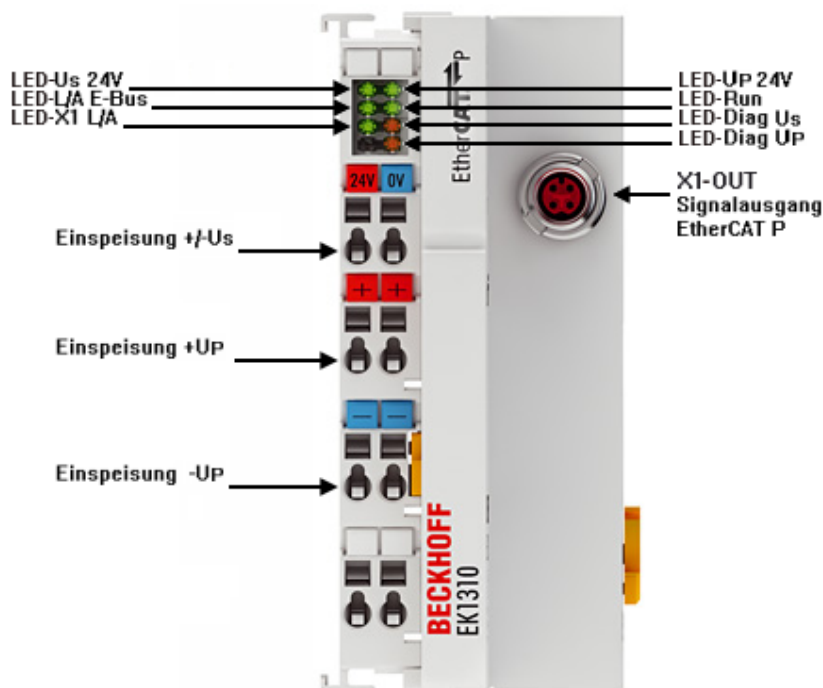
Abb. 47: EK1310 LEDs
