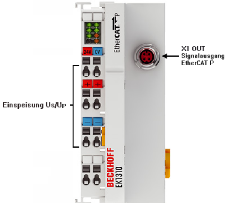
Abb. 10: EK1310
