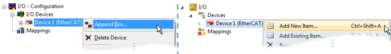
Fig. 136: Appending EtherCAT devices (left: TwinCAT 2; right: TwinCAT 3)
