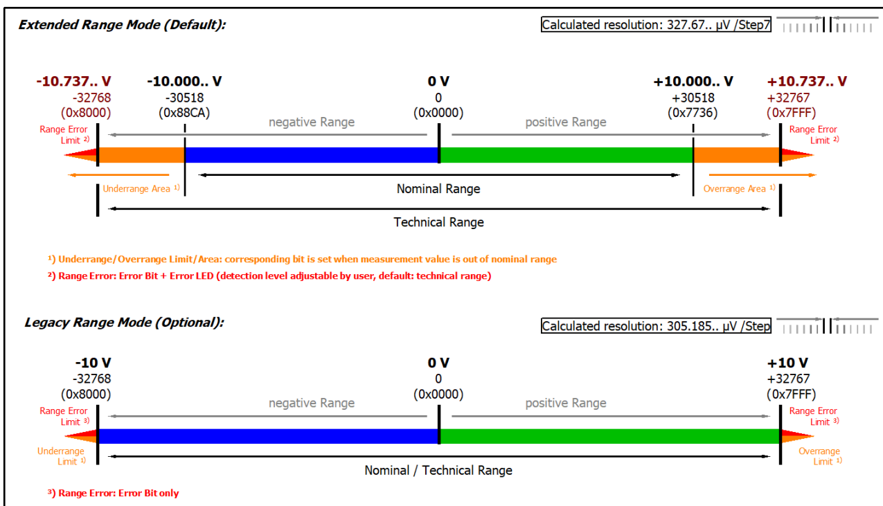
Fig. 200: EL3072, EL3074; measuring range -10...+10 V
