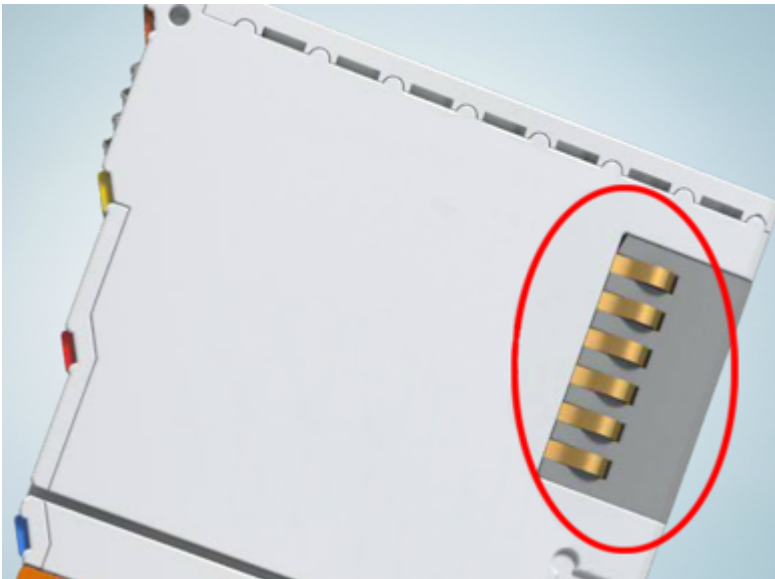
Fig. 90: Spring contacts of the Beckhoff I/O components
