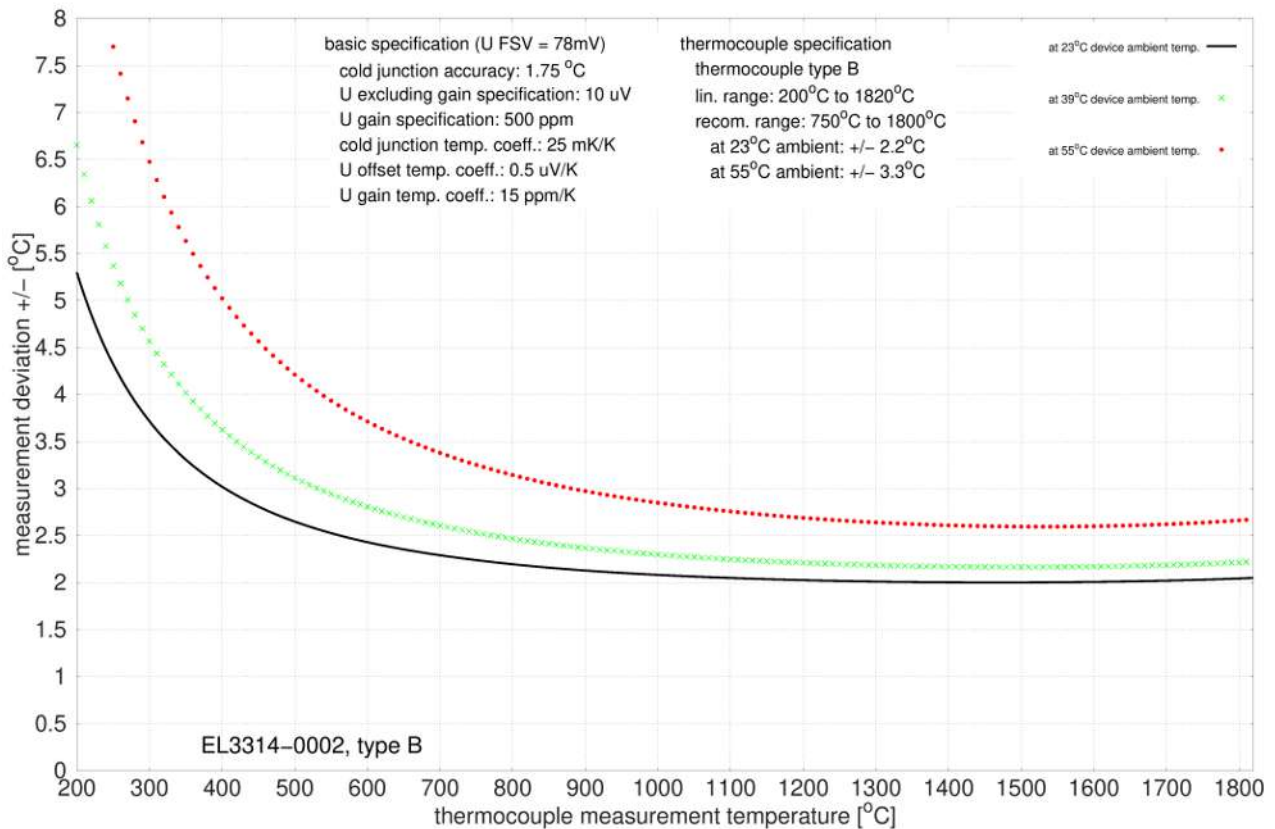
Fig. 11: EL3314-0002 and EL3314-0092 (corresponds to EL3314-0002), type B
