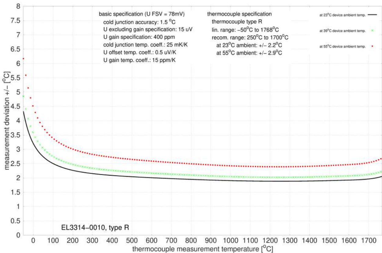
Fig. 44: EL3314-0010, EL3314-0020 and EL3314-0030 (equivalent to EL3314-0010), type R
