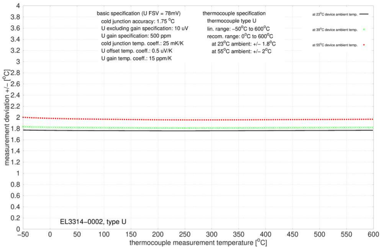
Fig. 75: EL3314-0002 and EL3314-0092 (corresponds to EL3314-0002), type U
