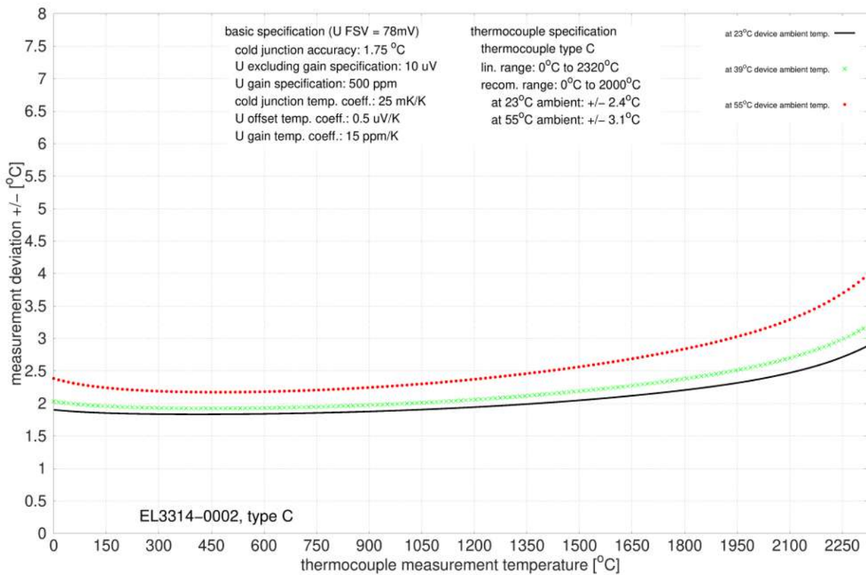
Fig. 12: EL3314-0002 and EL3314-0092 (corresponds to EL3314-0002), type C
