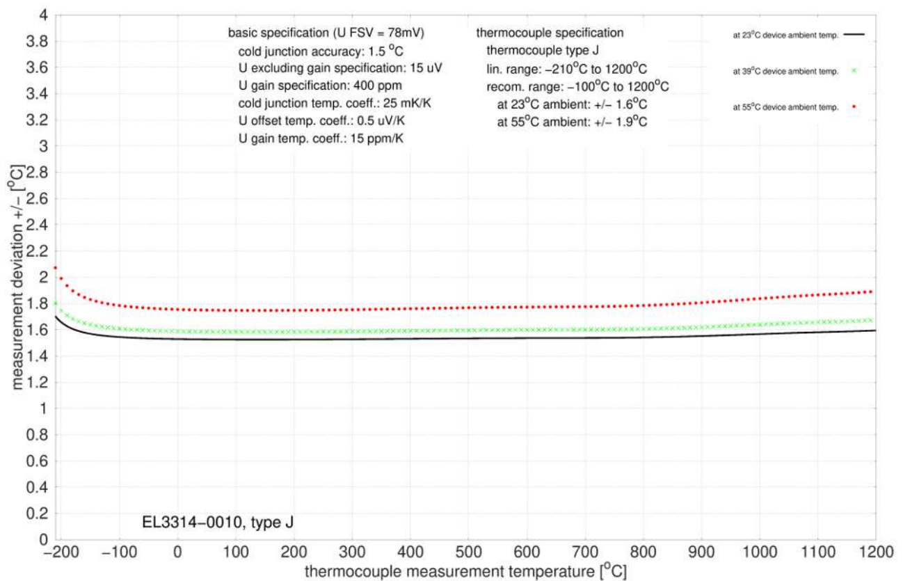
Fig. 40: EL3314-0010, EL3314-0020 and EL3314-0030 (equivalent to EL3314-0010), type J
