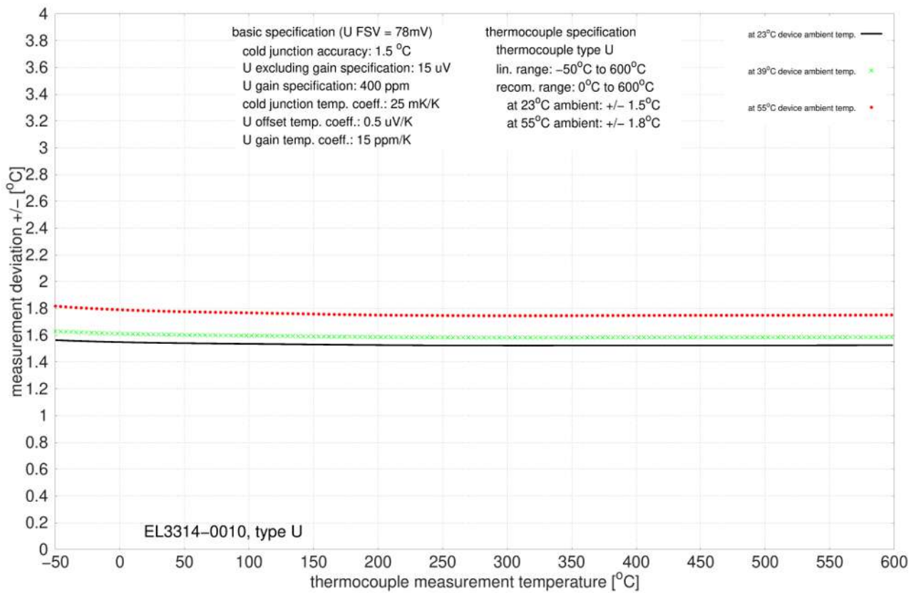
Fig. 34: EL3314-0010, EL3314-0020 and EL3314-0030 (equivalent to EL3314-0010), type U
