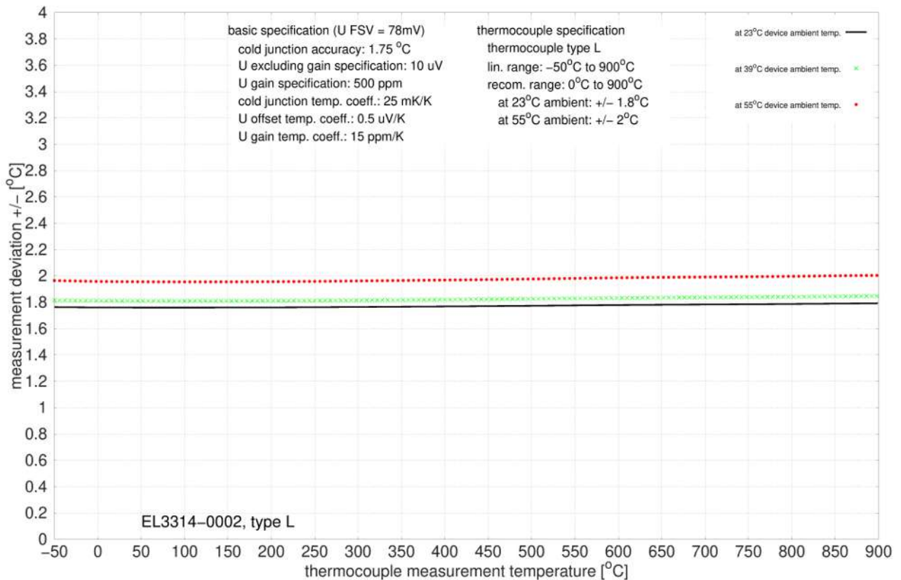
Fig. 70: EL3314-0002 and EL3314-0092 (corresponds to EL3314-0002), type L
