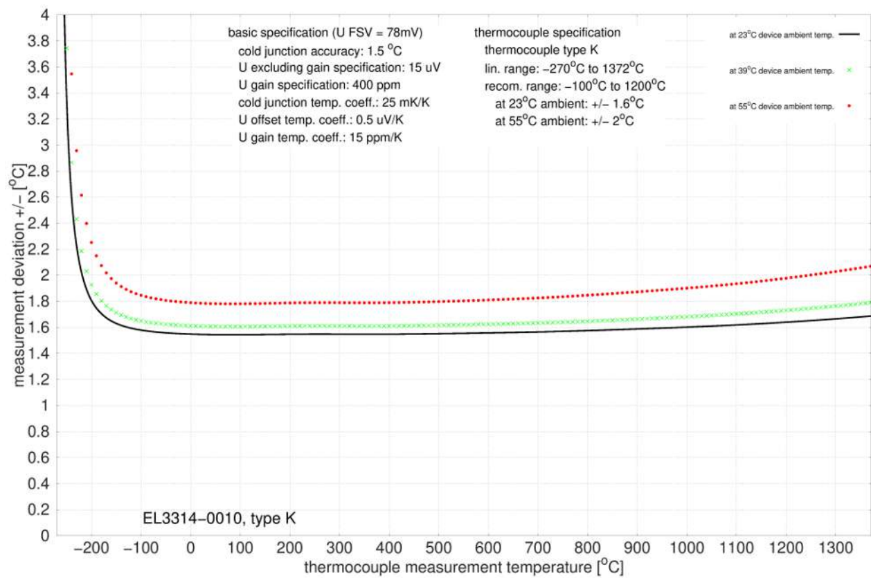
Fig. 28: EL3314-0010, EL3314-0020 and EL3314-0030 (equivalent to EL3314-0010), type K
