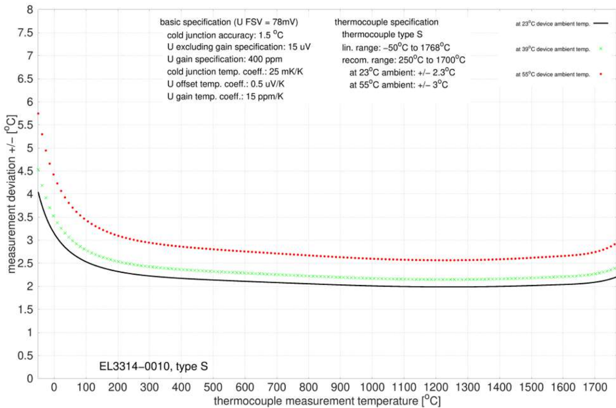
Fig. 58: EL3314-0010, EL3314-0020 and EL3314-0030 (equivalent to EL3314-0010), type S
