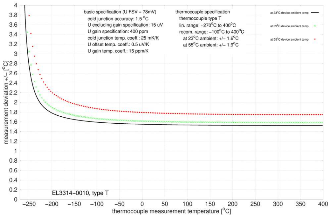
Fig. 46: EL3314-0010, EL3314-0020 and EL3314-0030 (equivalent to EL3314-0010), type T
