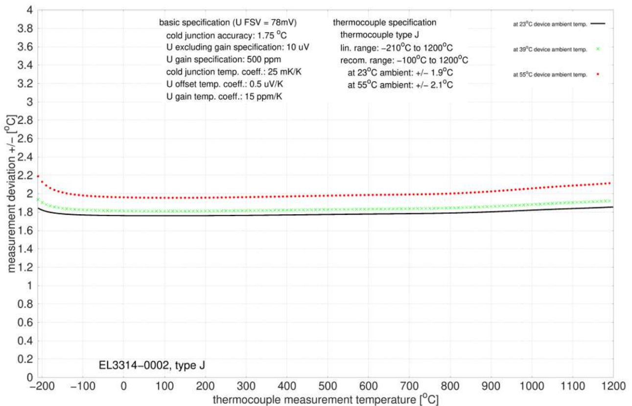
Fig. 14: EL3314-0002 and EL3314-0092 (corresponds to EL3314-0002), type J
