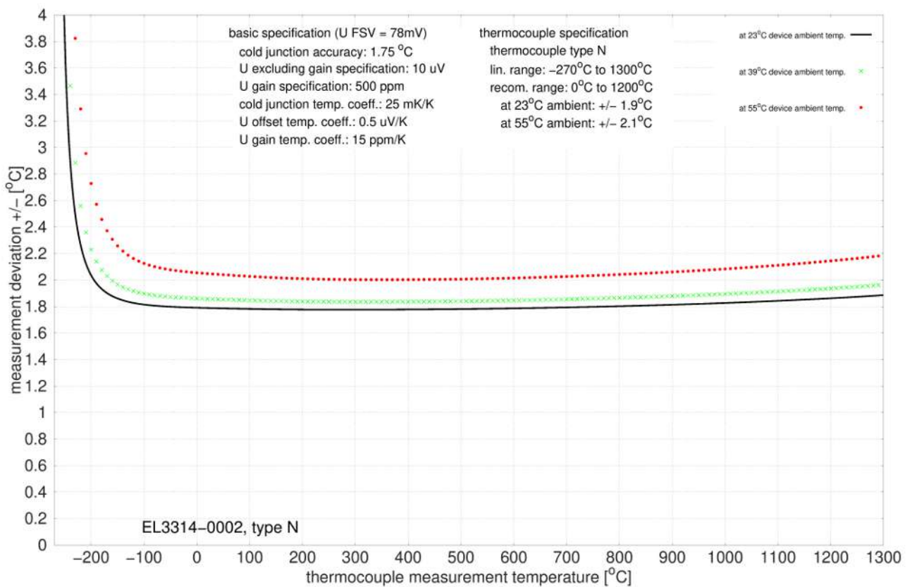
Fig. 17: EL3314-0002 and EL3314-0092 (corresponds to EL3314-0002), type N
