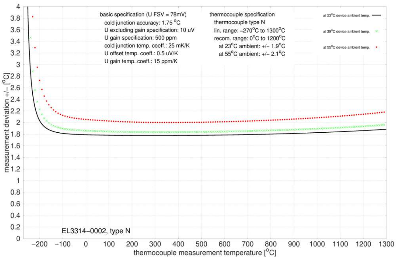
Fig. 71: EL3314-0002 and EL3314-0092 (corresponds to EL3314-0002), type N
