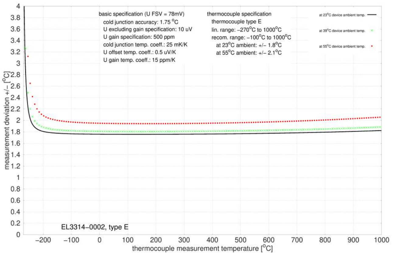
Fig. 67: EL3314-0002 and EL3314-0092 (corresponds to EL3314-0002), type E
