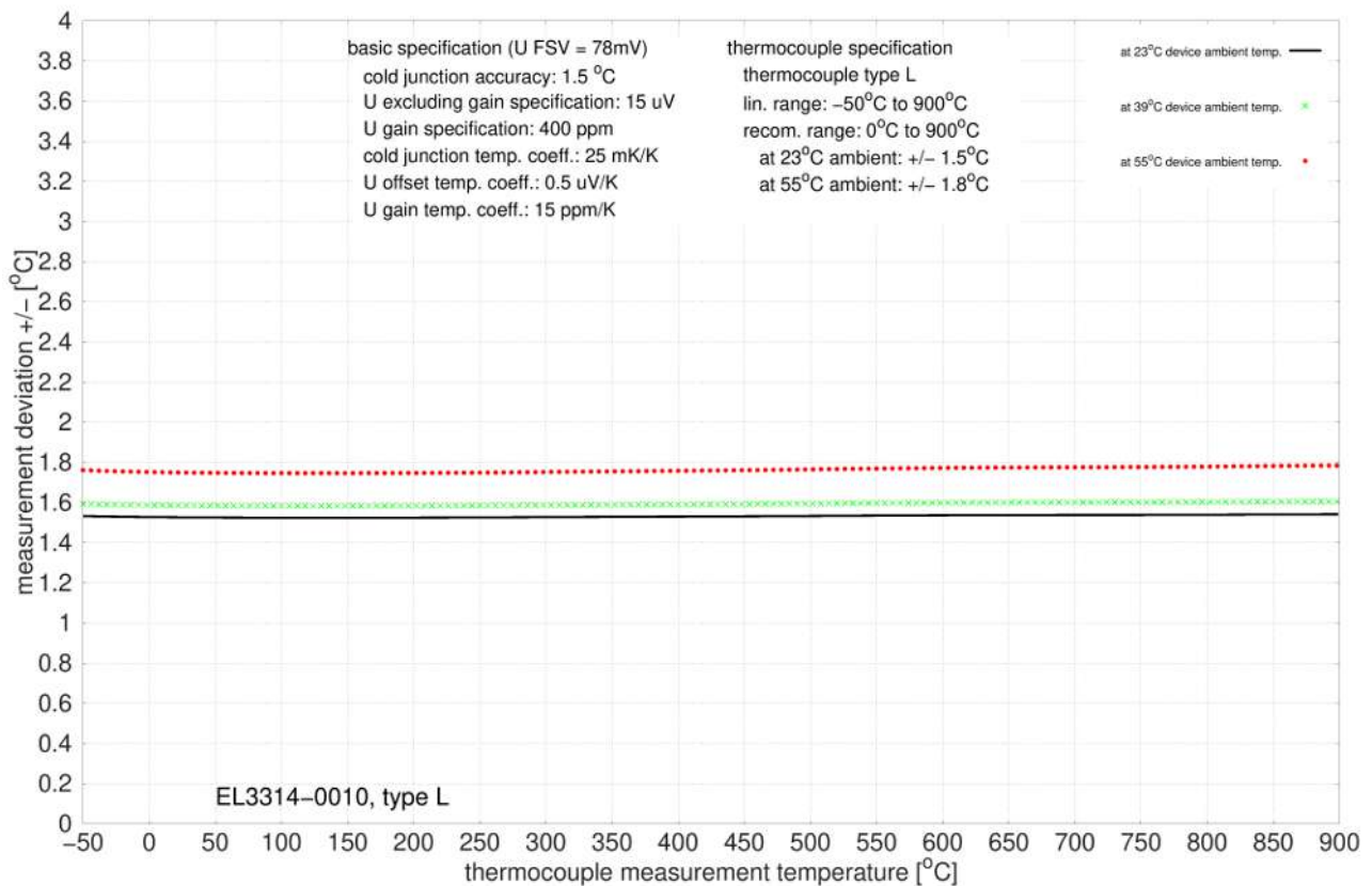
Fig. 29: EL3314-0010, EL3314-0020 and EL3314-0030 (equivalent to EL3314-0010), type L
