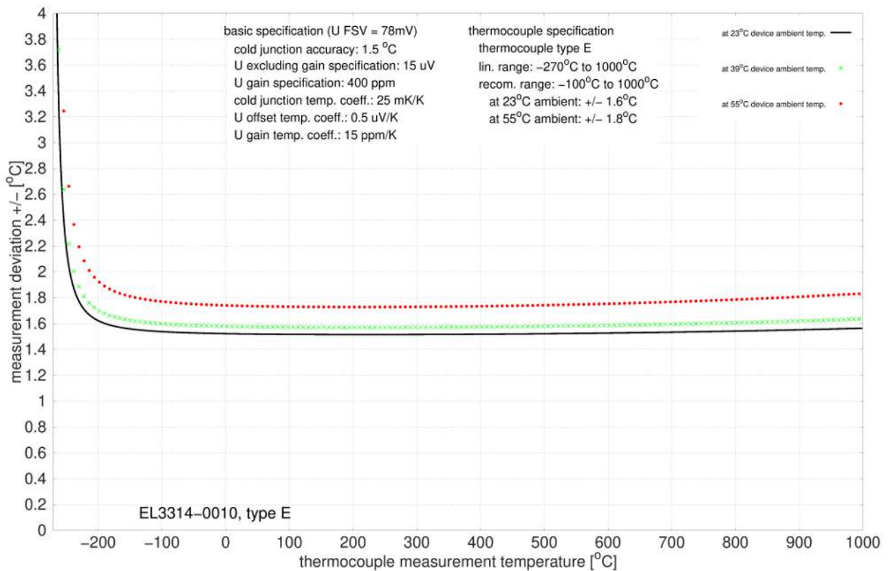
Fig. 26: EL3314-0010, EL3314-0020 and EL3314-0030 (equivalent to EL3314-0010), type E
