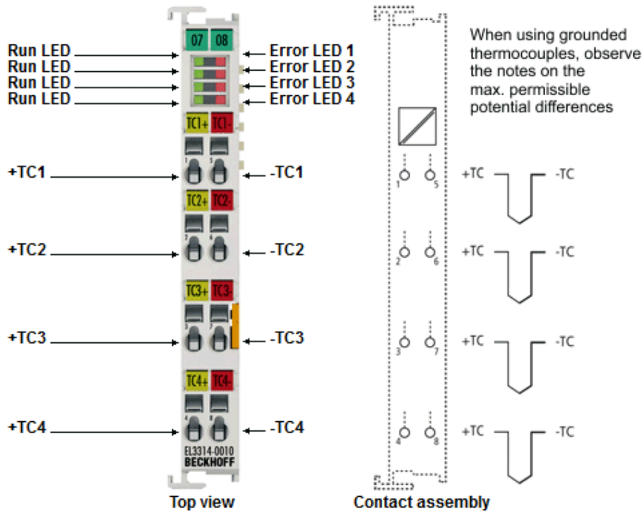
Fig. 48: EL3314-0020 (corresponds to EL3314-0010)
