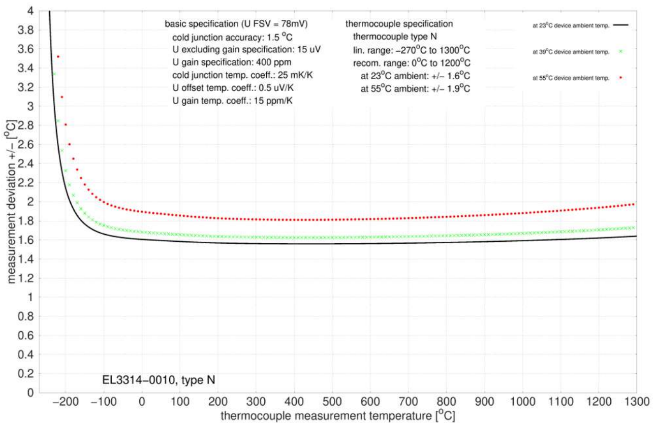
Fig. 30: EL3314-0010, EL3314-0020 and EL3314-0030 (equivalent to EL3314-0010), type N
