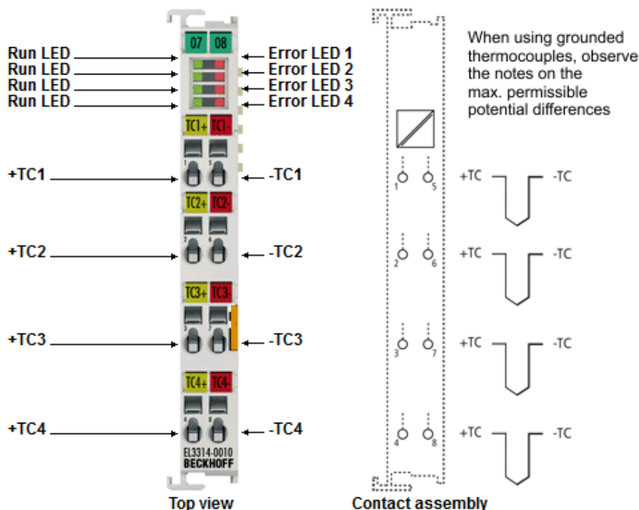
Fig. 36: EL3314-0020 (corresponds to EL3314-0010)
