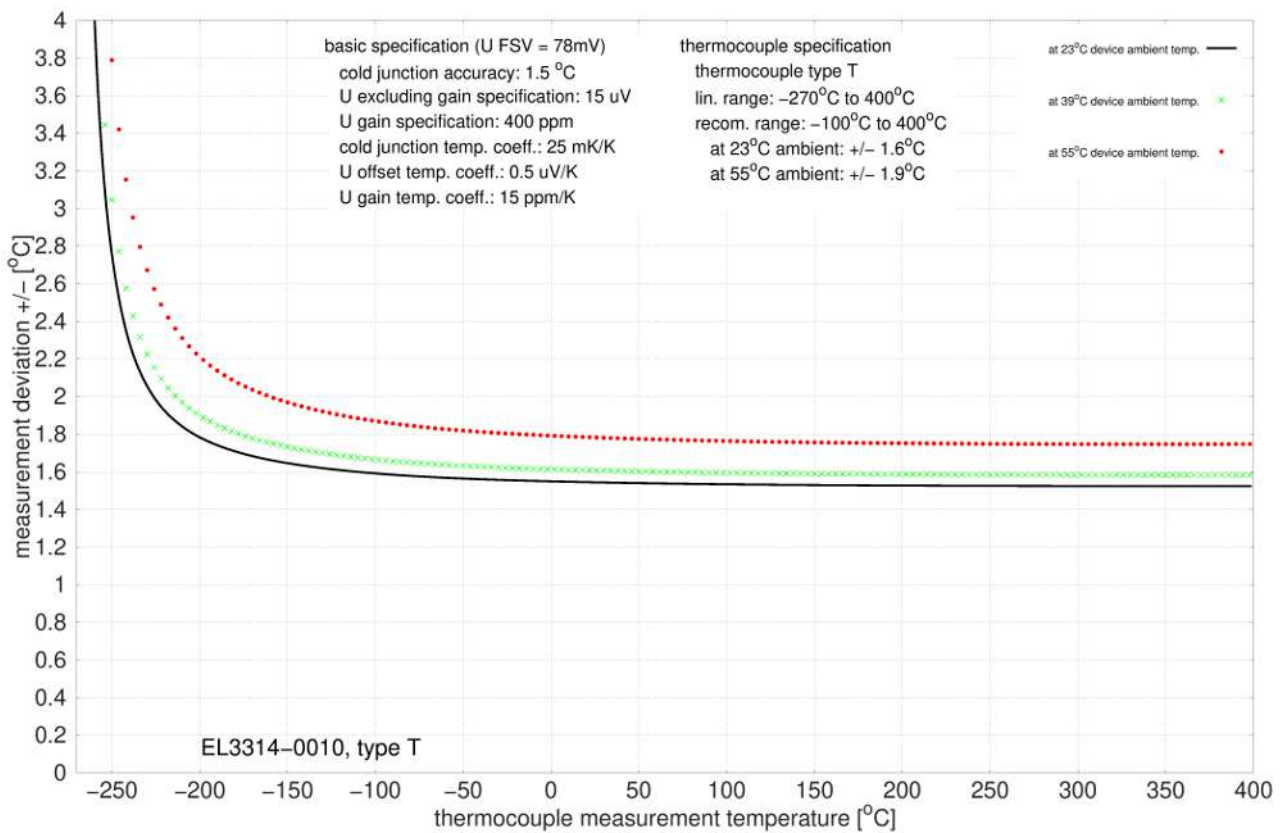
Fig. 33: EL3314-0010, EL3314-0020 and EL3314-0030 (equivalent to EL3314-0010), type T
