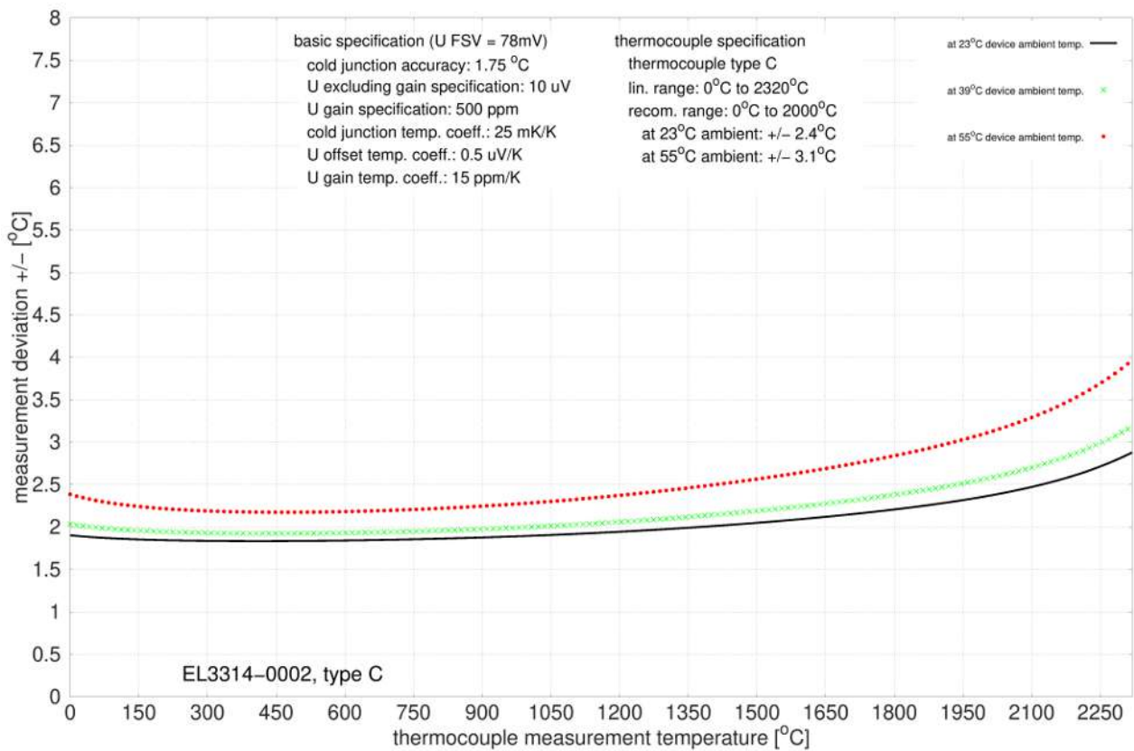
Fig. 66: EL3314-0002 and EL3314-0092 (corresponds to EL3314-0002), type C
