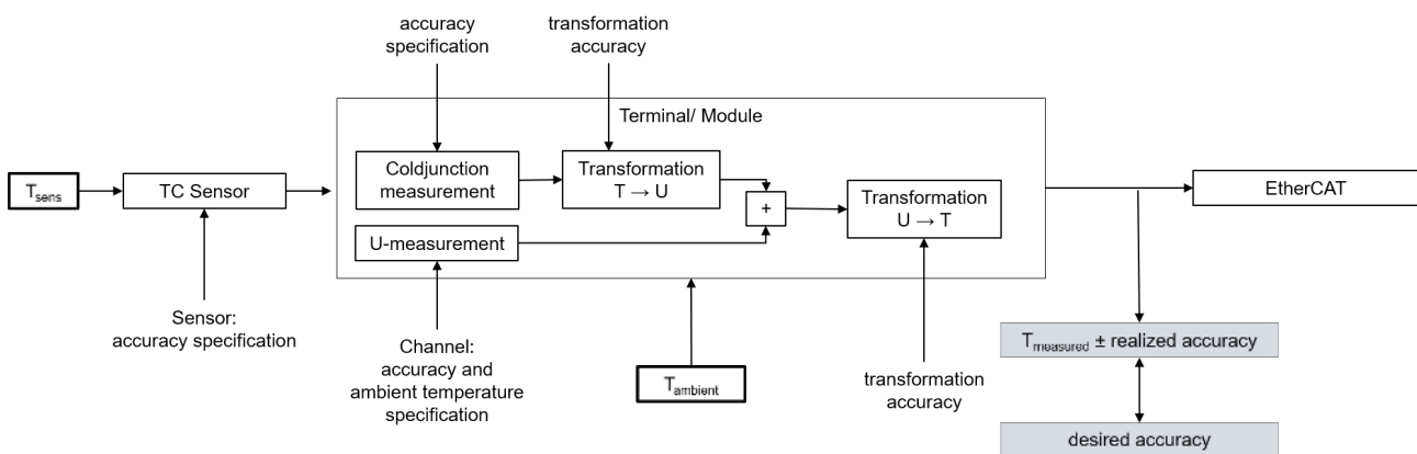
Fig. 80: Concatenation of the uncertainties in temperature measurement with thermocouples
