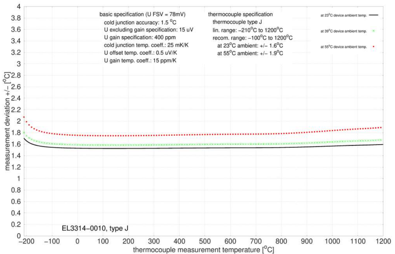
Fig. 53: EL3314-0010, EL3314-0020 and EL3314-0030 (equivalent to EL3314-0010), type J
