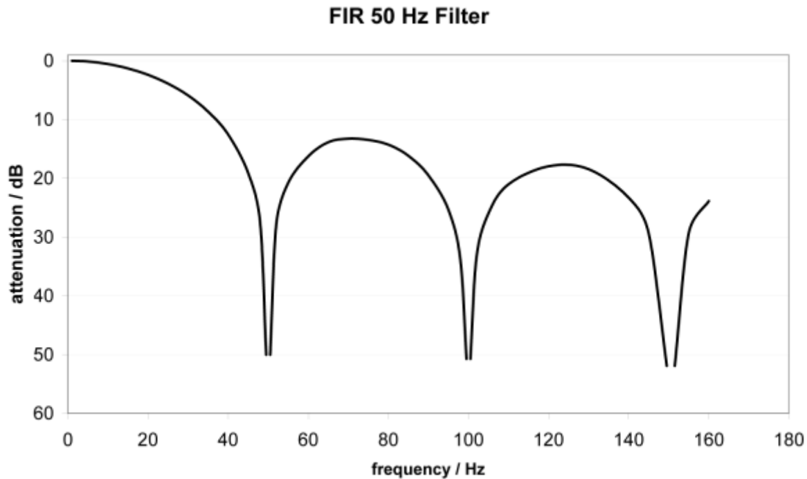
Fig. 226: Example notch filter
