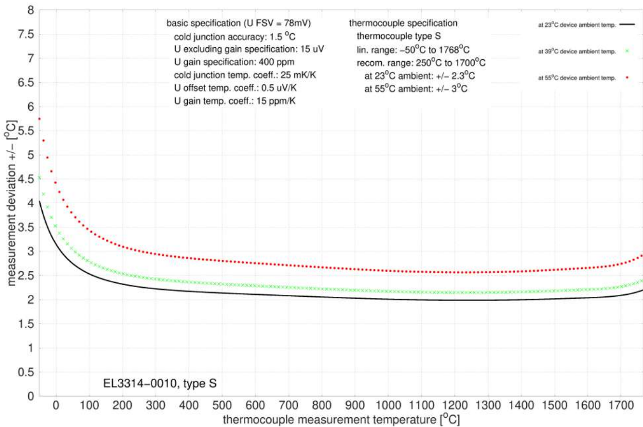
Fig. 45: EL3314-0010, EL3314-0020 and EL3314-0030 (equivalent to EL3314-0010), type S
