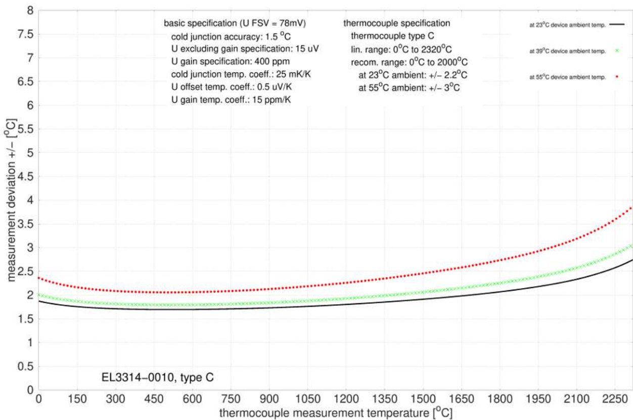
Fig. 38: EL3314-0010, EL3314-0020 and EL3314-0030 (equivalent to EL3314-0010), type C
