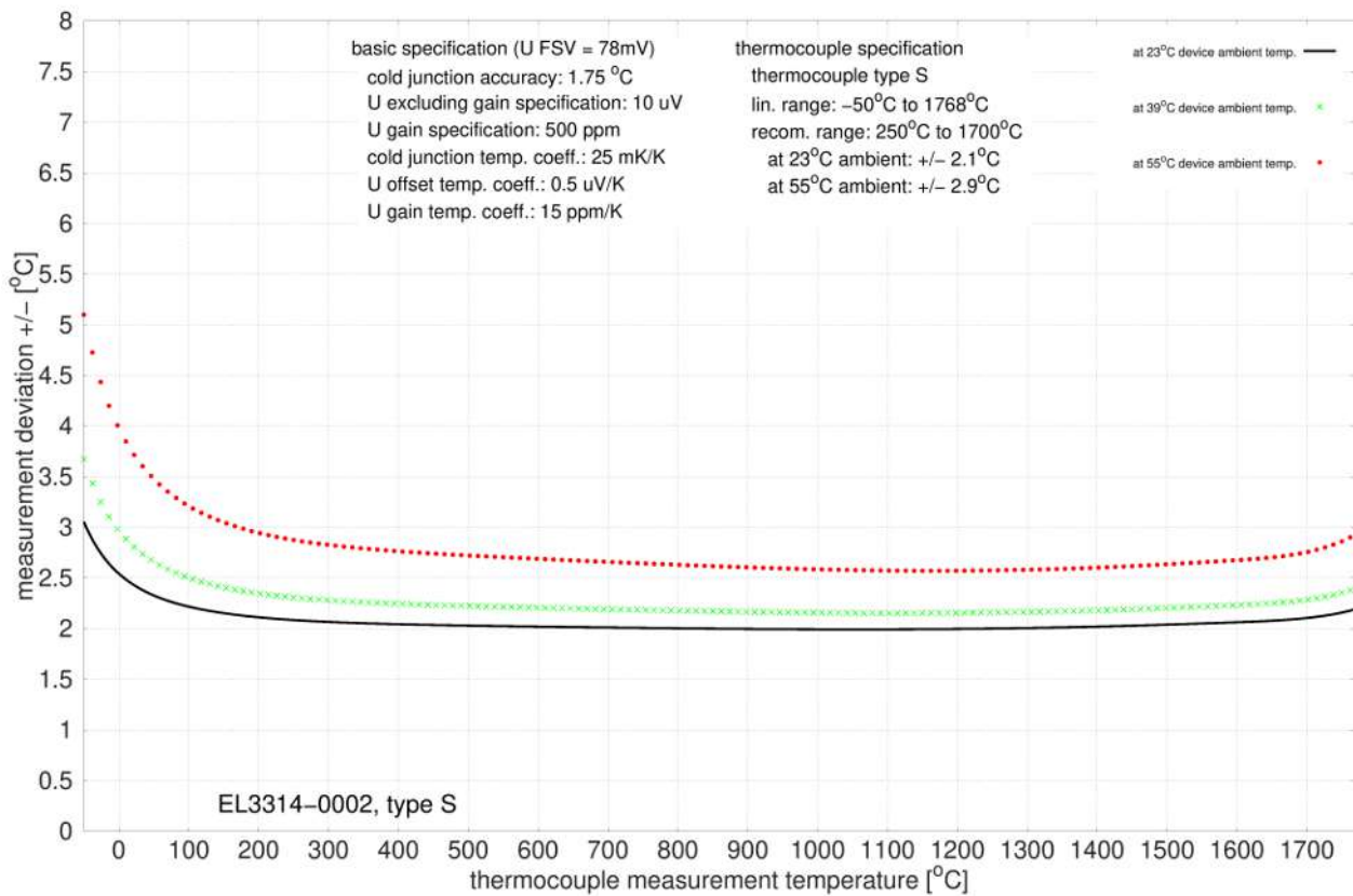
Fig. 19: EL3314-0002 and EL3314-0092 (corresponds to EL3314-0002), type S
