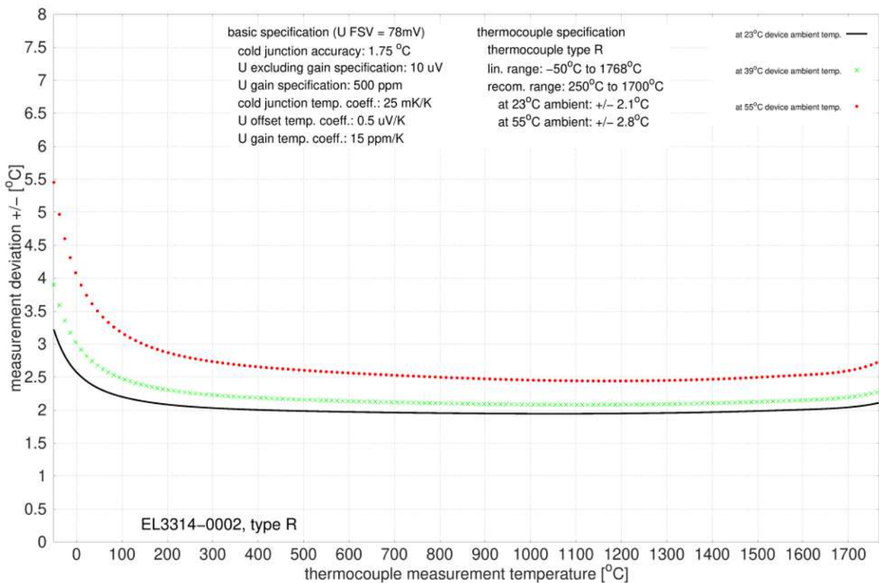
Fig. 18: EL3314-0002 and EL3314-0092 (corresponds to EL3314-0002), type R
