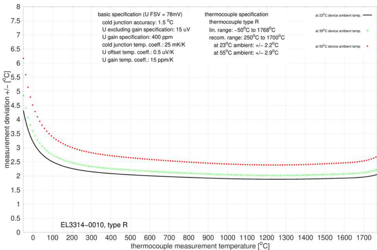
Fig. 31: EL3314-0010, EL3314-0020 and EL3314-0030 (equivalent to EL3314-0010), type R
