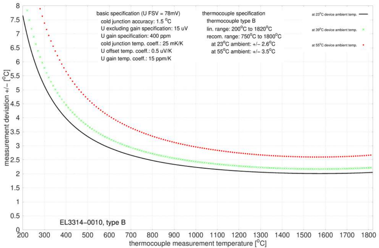
Fig. 37: EL3314-0010, EL3314-0020 and EL3314-0030 (equivalent to EL3314-0010), type B
