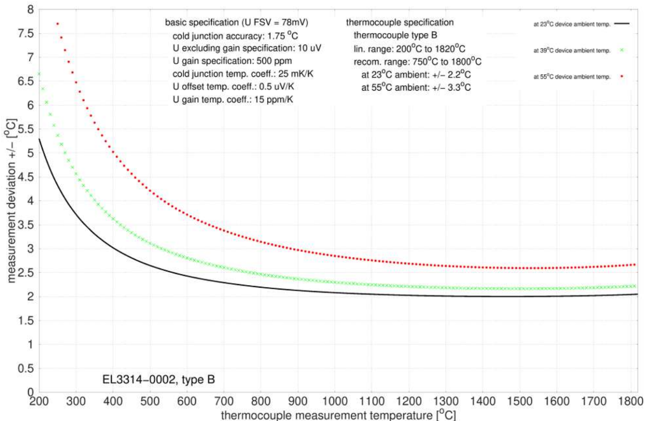
Fig. 65: EL3314-0002 and EL3314-0092 (corresponds to EL3314-0002), type B
