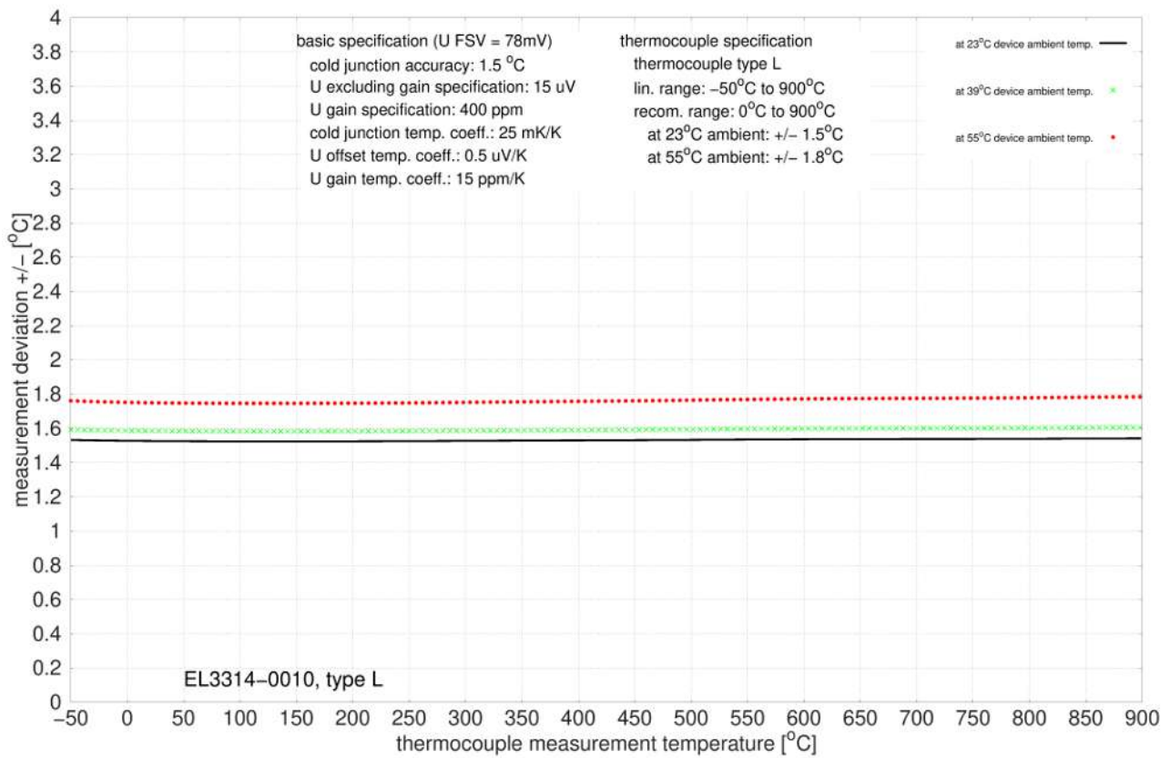
Fig. 42: EL3314-0010, EL3314-0020 and EL3314-0030 (equivalent to EL3314-0010), type L
