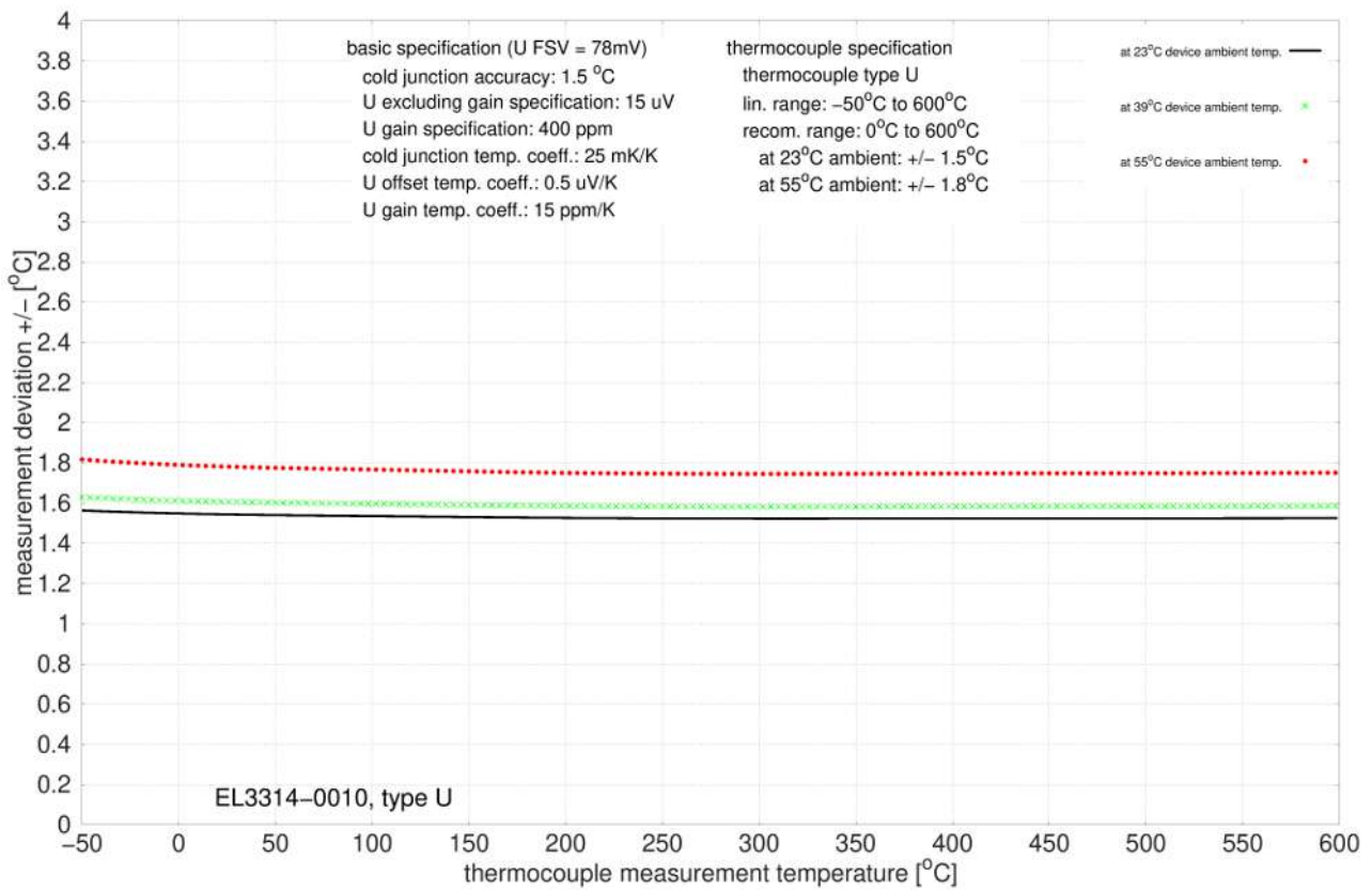
Fig. 47: EL3314-0010, EL3314-0020 and EL3314-0030 (equivalent to EL3314-0010), type U
