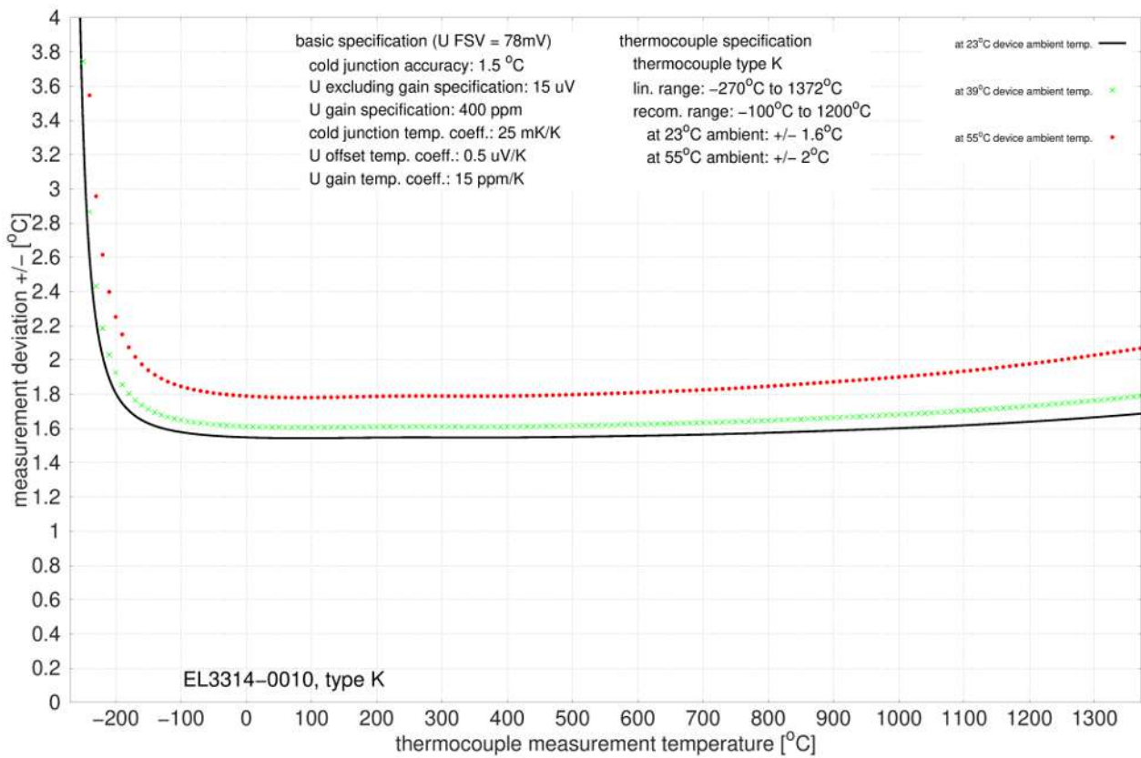
Fig. 41: EL3314-0010, EL3314-0020 and EL3314-0030 (equivalent to EL3314-0010), type K
