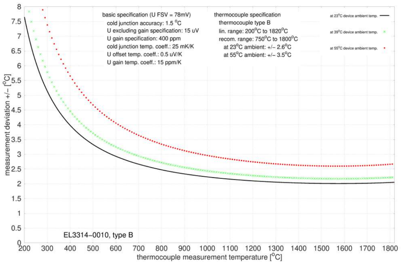
Fig. 24: EL3314-0010, EL3314-0020 and EL3314-0030 (equivalent to EL3314-0010), type B
