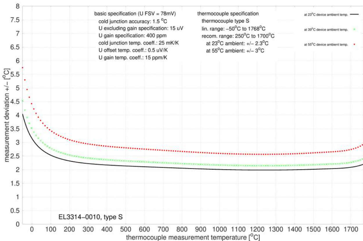
Fig. 32: EL3314-0010, EL3314-0020 and EL3314-0030 (equivalent to EL3314-0010), type S
