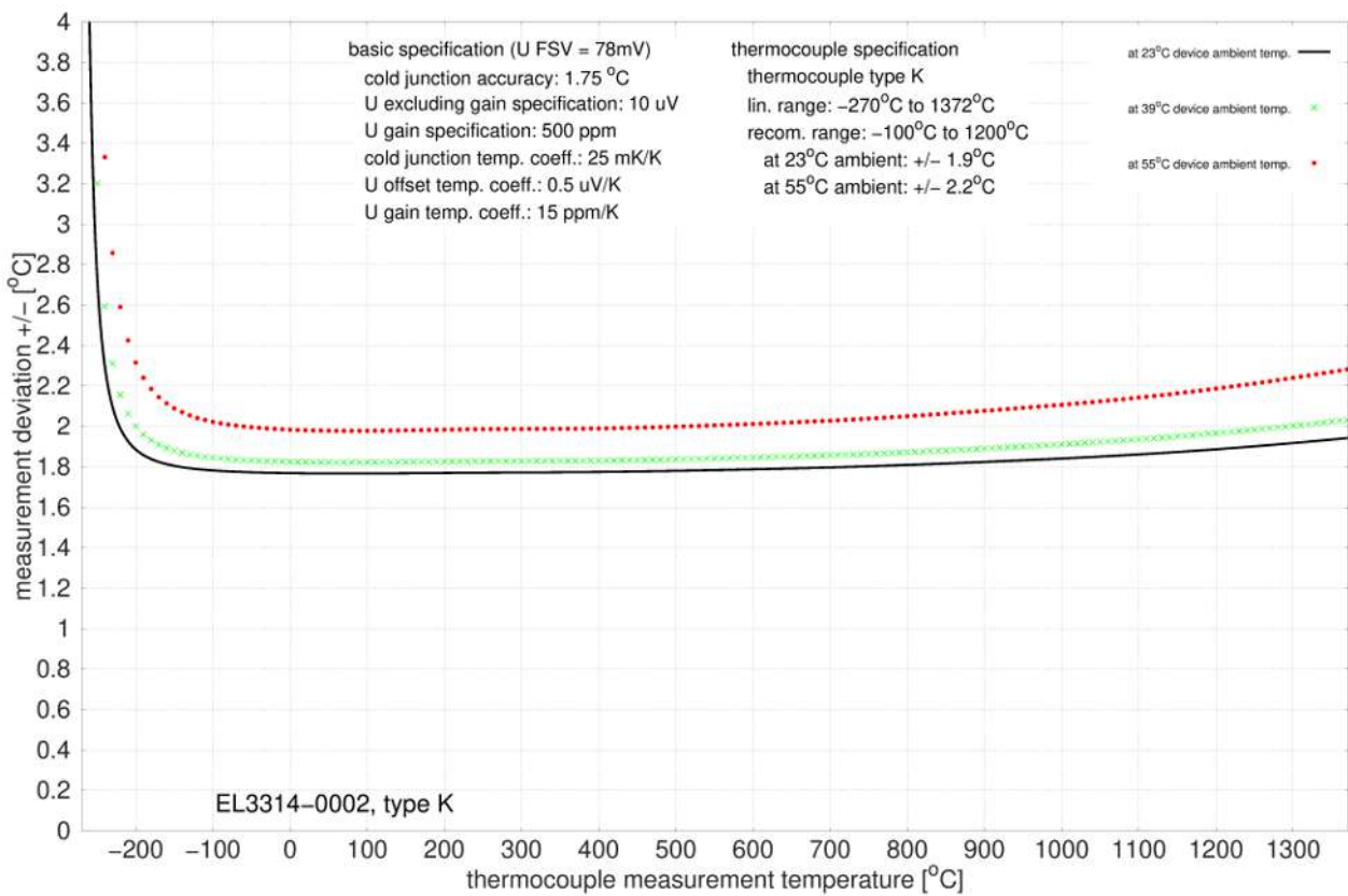
Fig. 15: EL3314-0002 and EL3314-0092 (corresponds to EL3314-0002), type K
