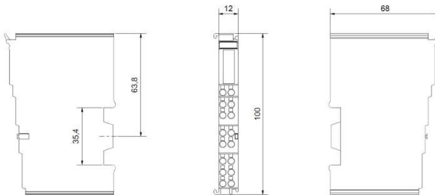
Fig. 78: Technical drawing | housing EL-12-16 pin
