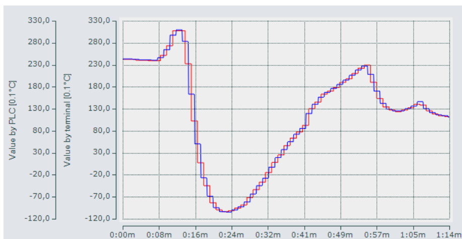
Fig. 241: Blue: temperature values from the PLC calculation; red: PDO values in the temperature measurement range
