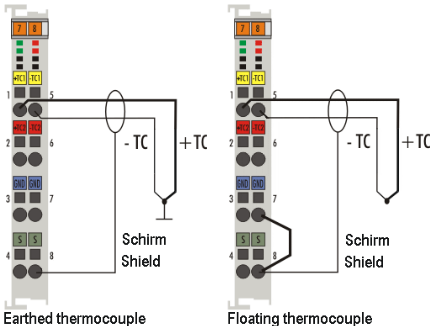
Fig. 98: Connection methods for earthed and earth-free thermocouples
