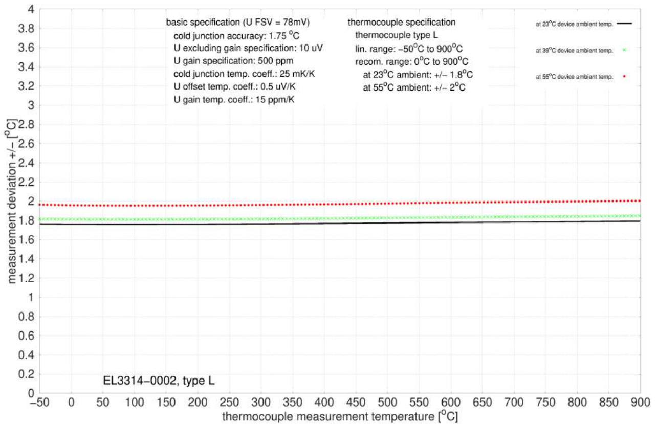
Fig. 16: EL3314-0002 and EL3314-0092 (corresponds to EL3314-0002), type L
