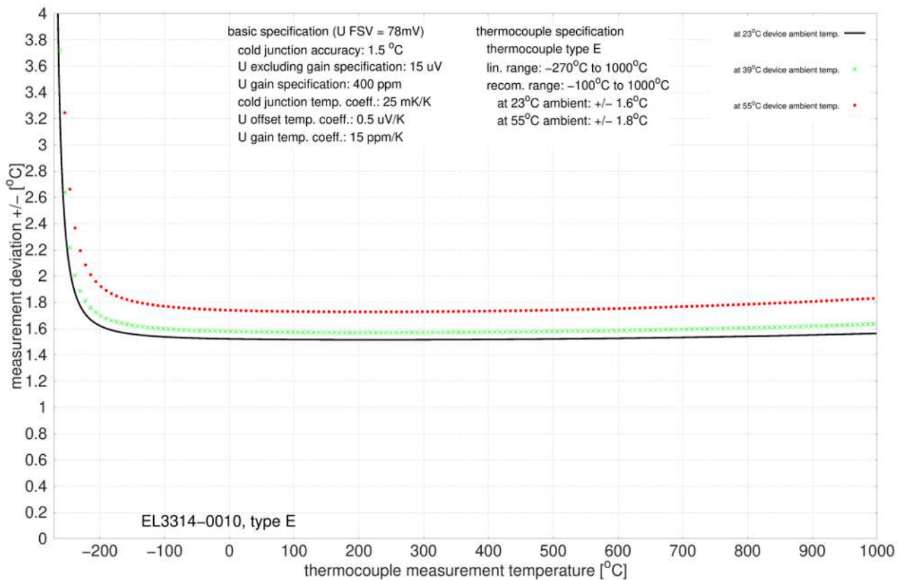
Fig. 39: EL3314-0010, EL3314-0020 and EL3314-0030 (equivalent to EL3314-0010), type E
