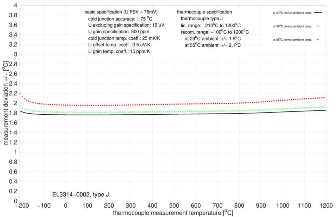
Fig. 68: EL3314-0002 and EL3314-0092 (corresponds to EL3314-0002), type J
