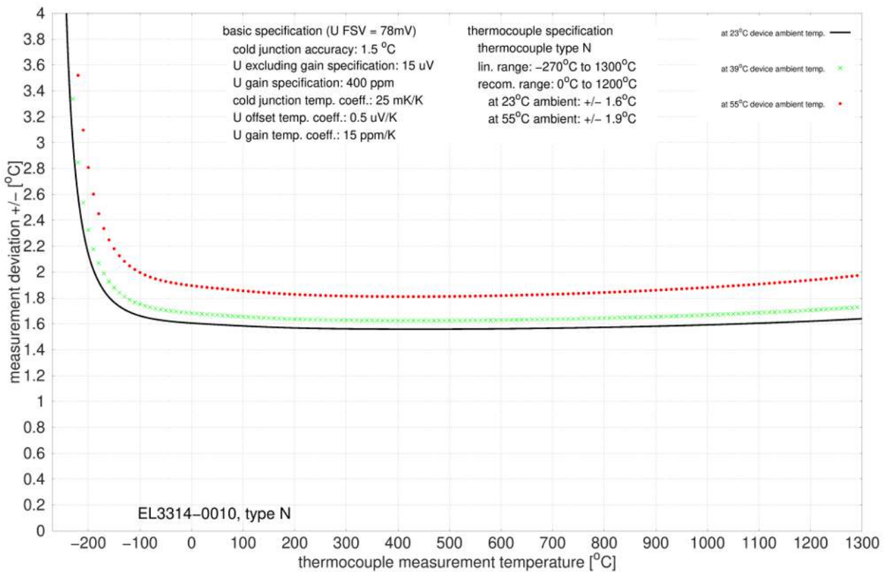
Fig. 43: EL3314-0010, EL3314-0020 and EL3314-0030 (equivalent to EL3314-0010), type N
