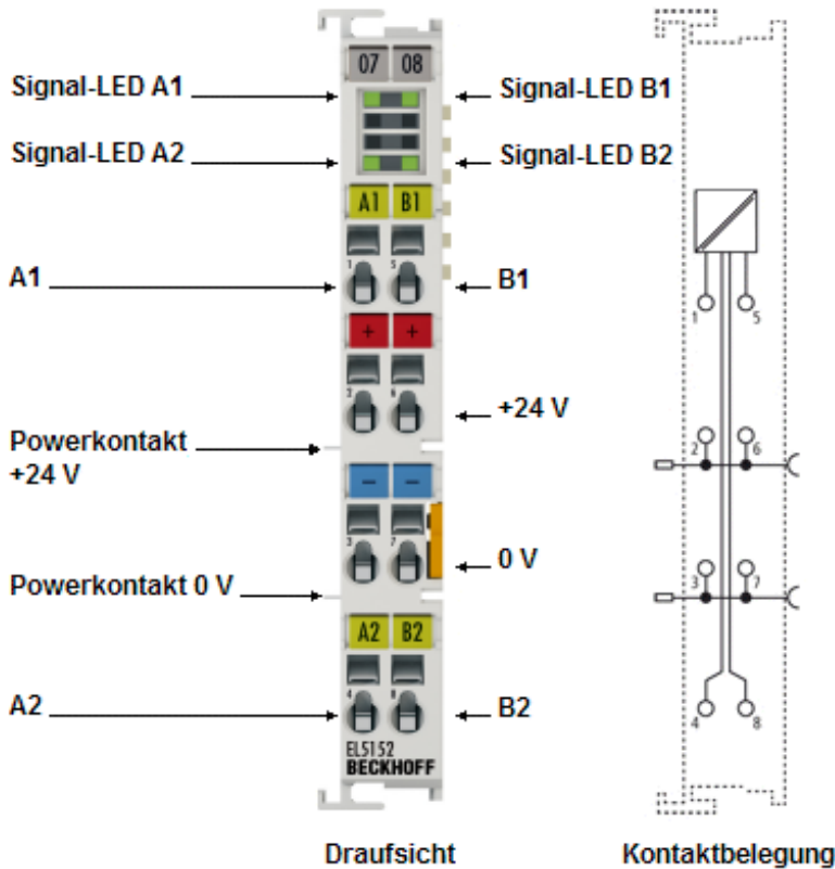
Abb. 7: EL5152
