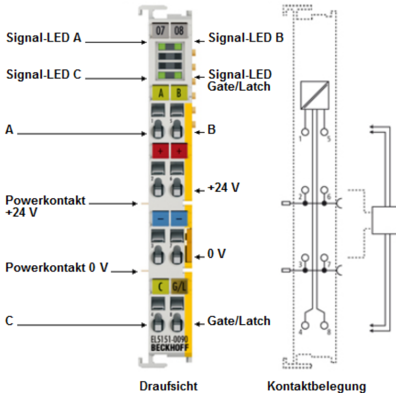
Abb. 6: EL5151-0090
