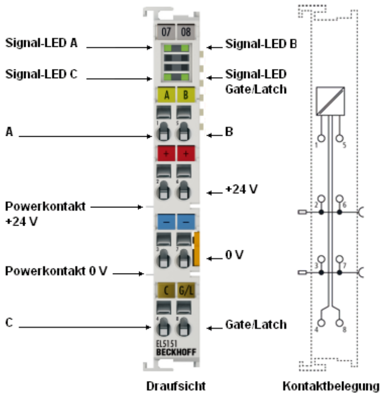
Abb. 4: EL5151
