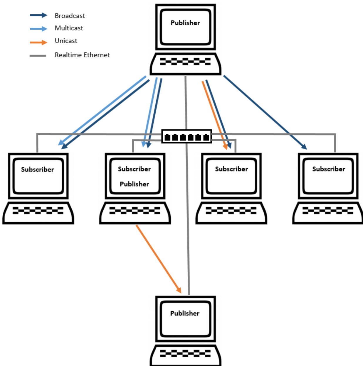
Abb. 110: Publisher/Subscriber Modell
