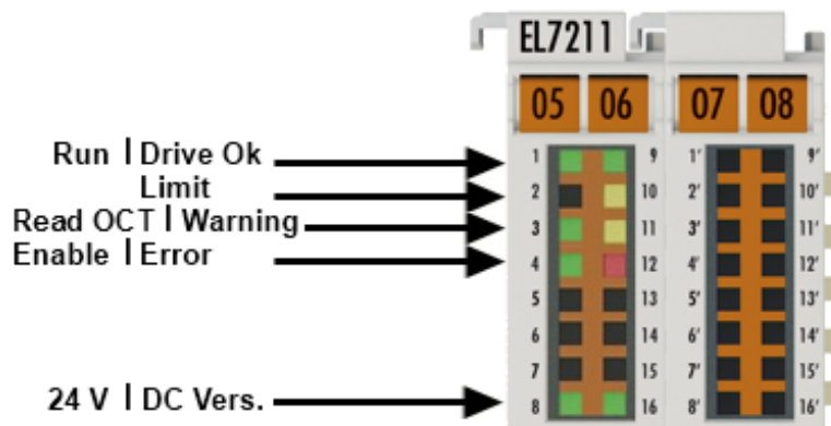
Abb. 36: EL7211-901x, EL7221-901x - LEDs
