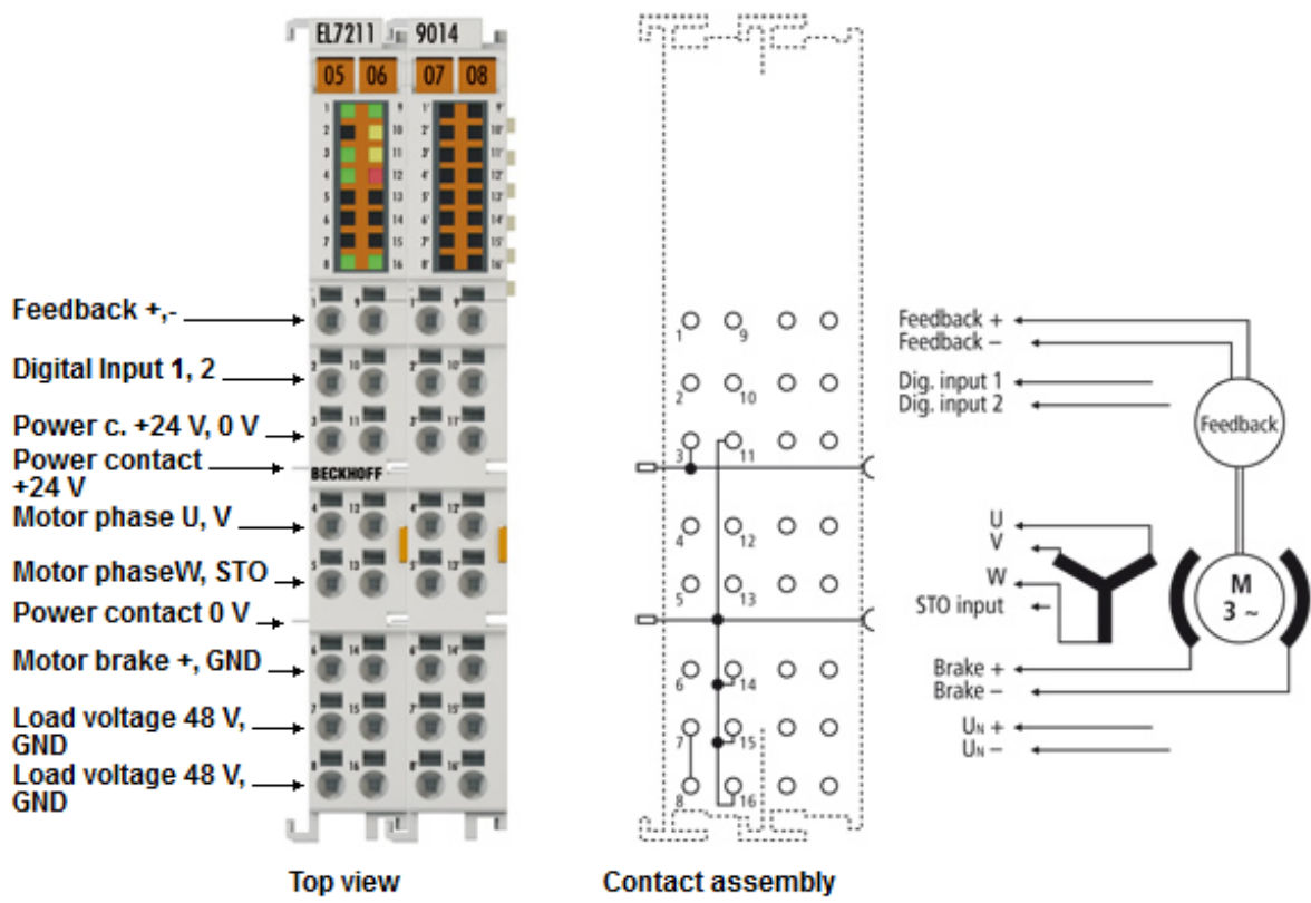
Abb. 5: EL7211-901x, EL7221-901x
