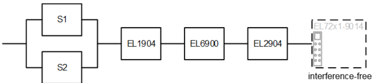
Abb. 214: EL72x1_9014_block_diagram
