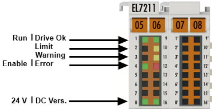
Abb. 35: EL7211, EL7211-0001 - LEDs
