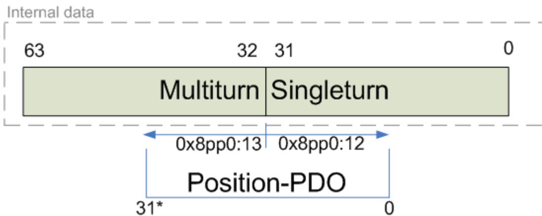
Abb. 114: Multiturn / Singleturn Bits
