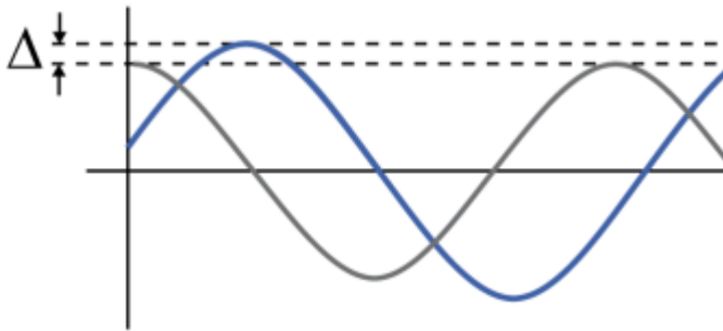
Abb. 115: Resolver gain adjustment
