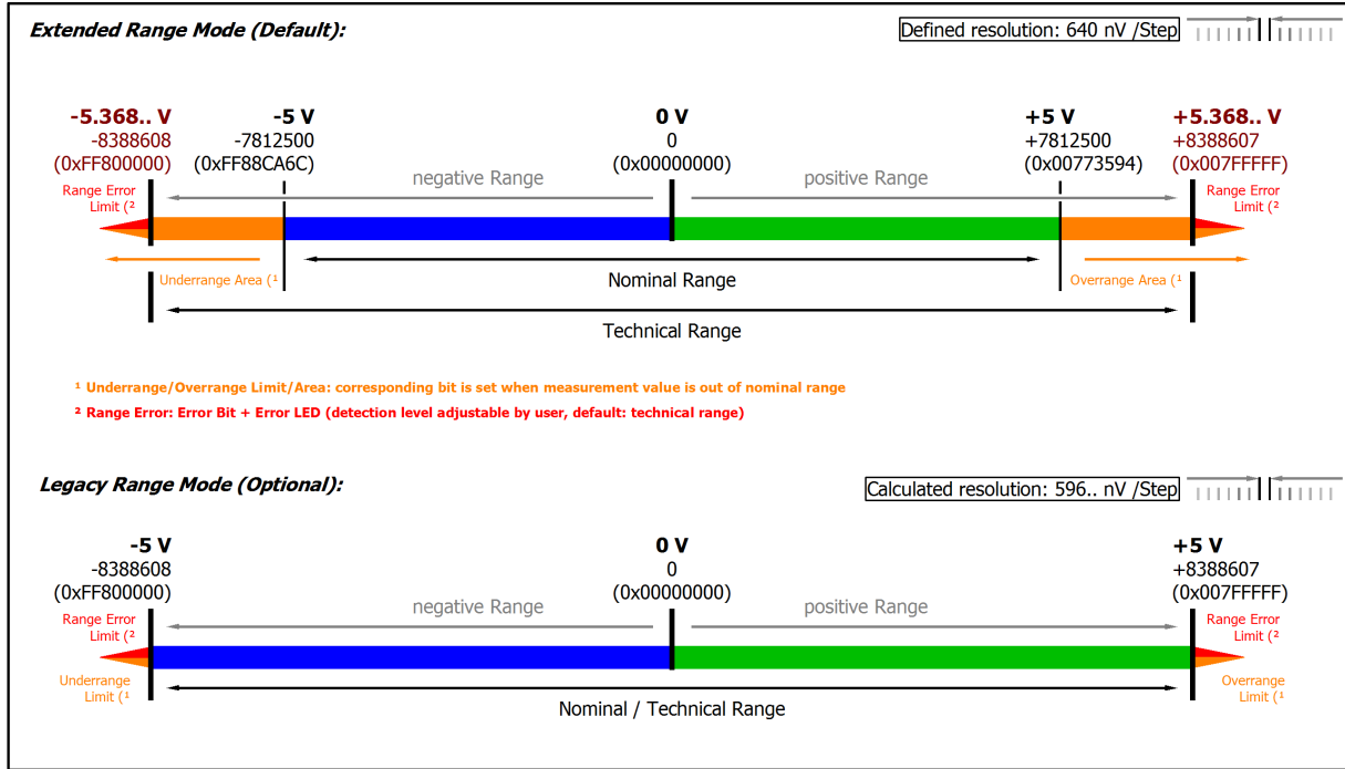
Fig. 55: Representation ±5 V measurement range
