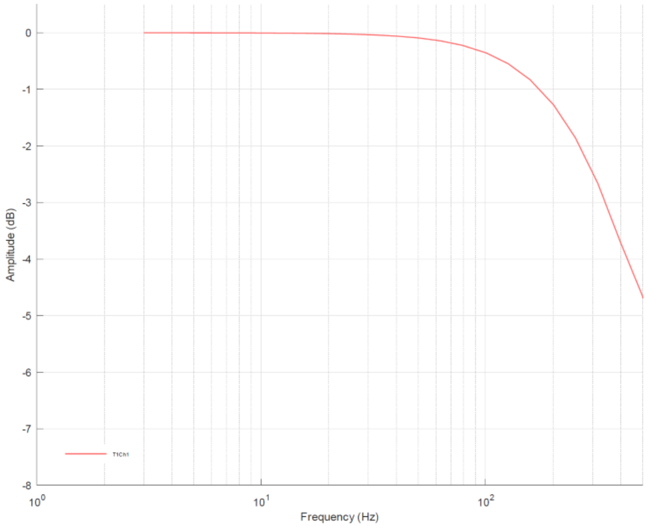
Fig. 60: Frequency response of measuring range \pm 2.5 V, f_{\text{sampling}} = 1 kHz, integrated filters 1/2 deactivated
