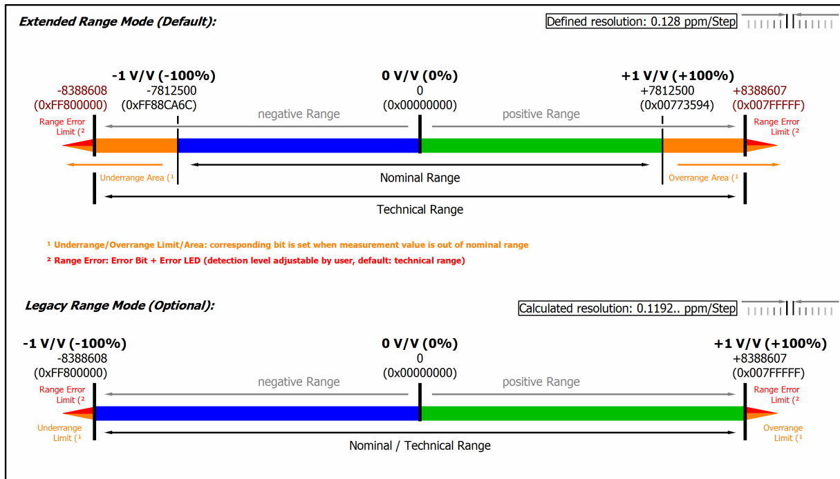
Fig. 182: Representation potentiometer measurement range
