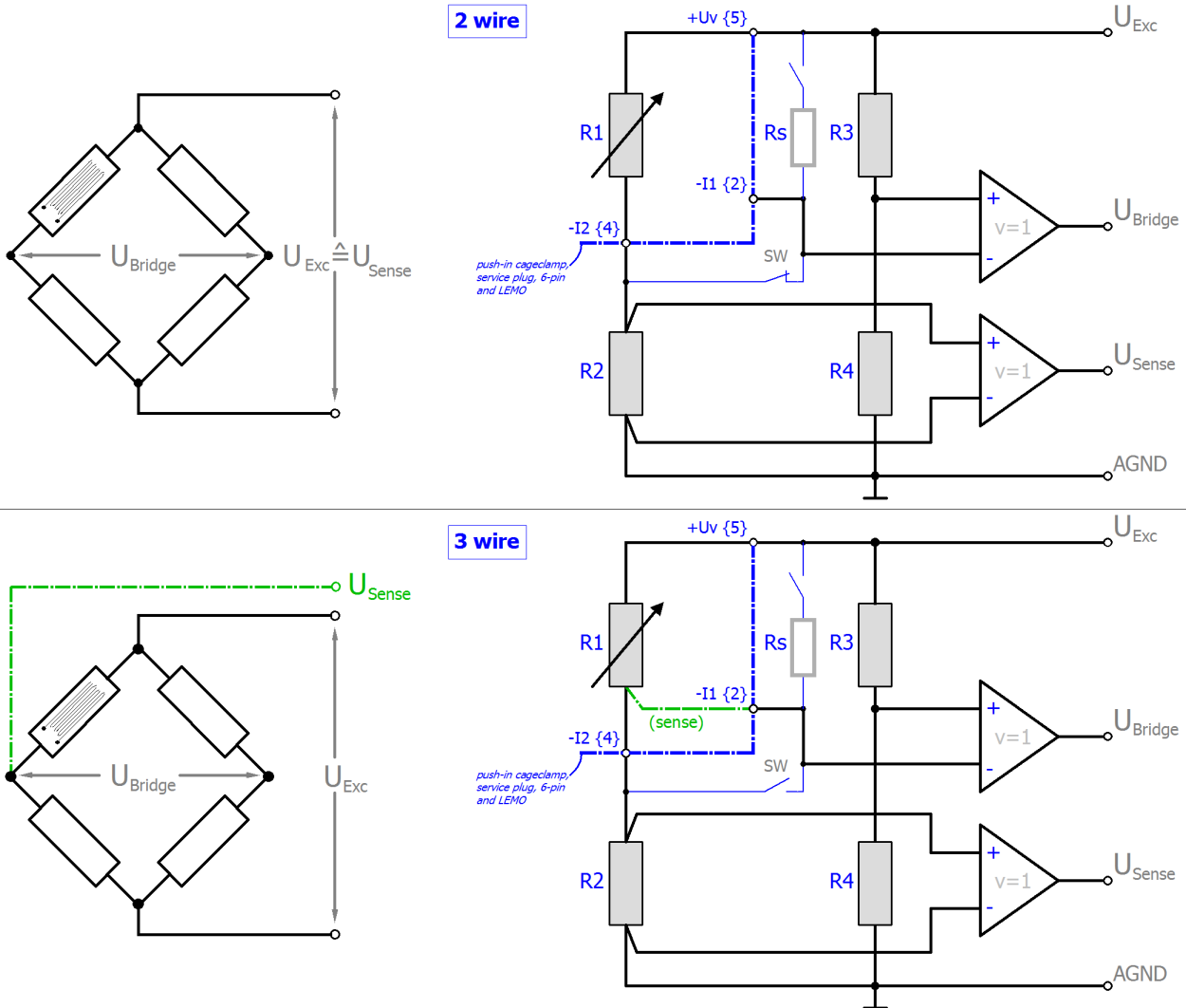
Fig. 142: Connection of the quarter bridge
