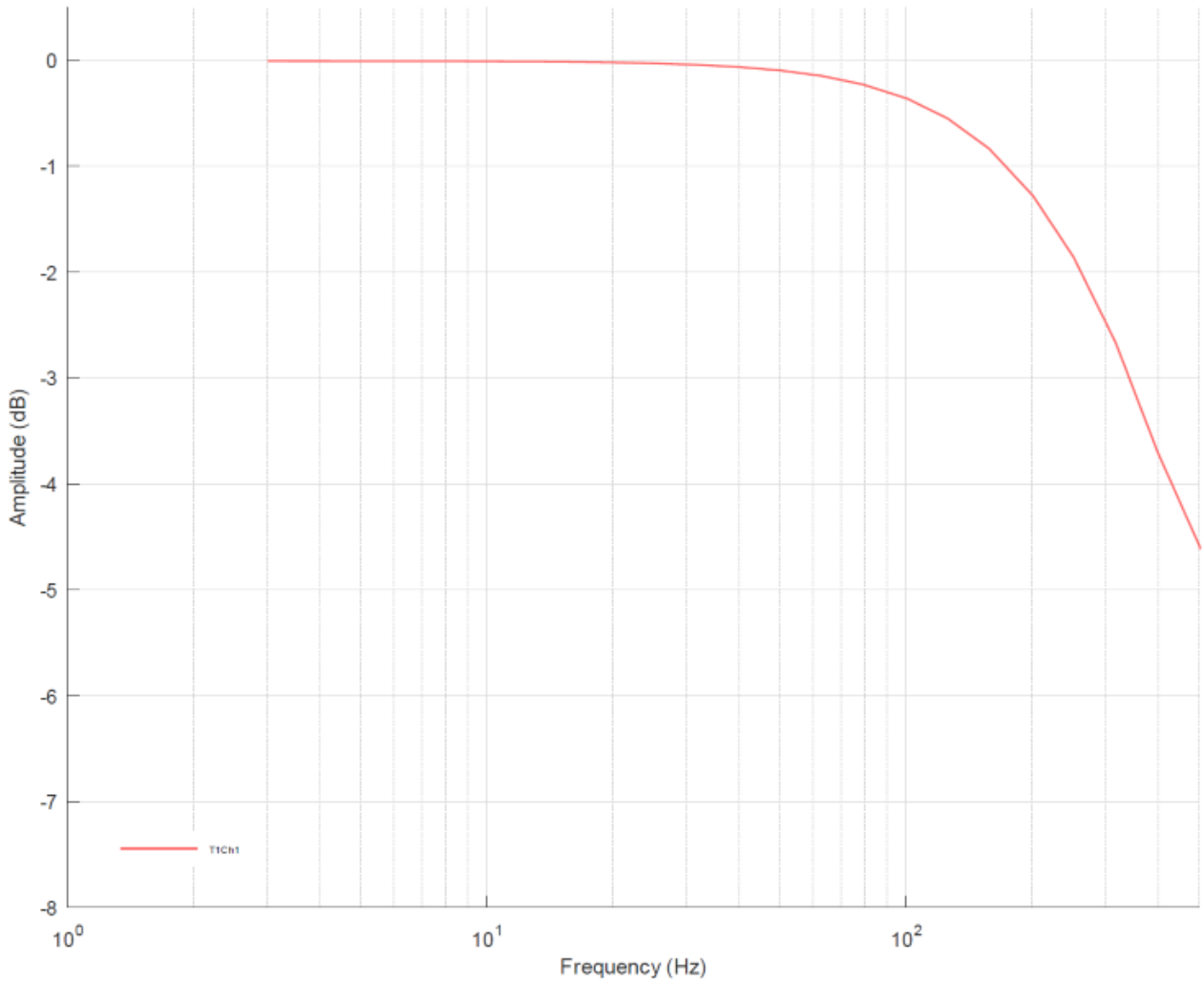
Fig. 62: Frequency response of measuring range \pm 1.25 V, f_{\text{sampling}} = 1 kHz, integrated filters 1/2 deactivated
