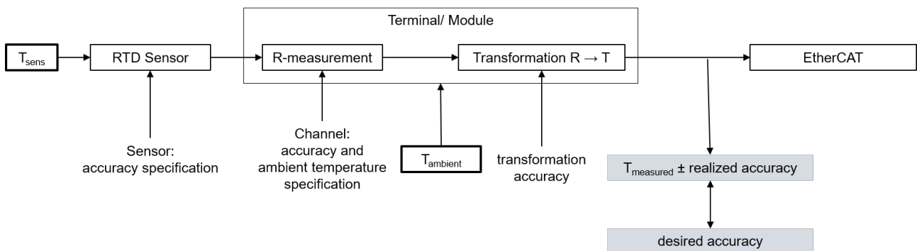
Fig. 84: Concatenation of the uncertainties in RTD measurement
