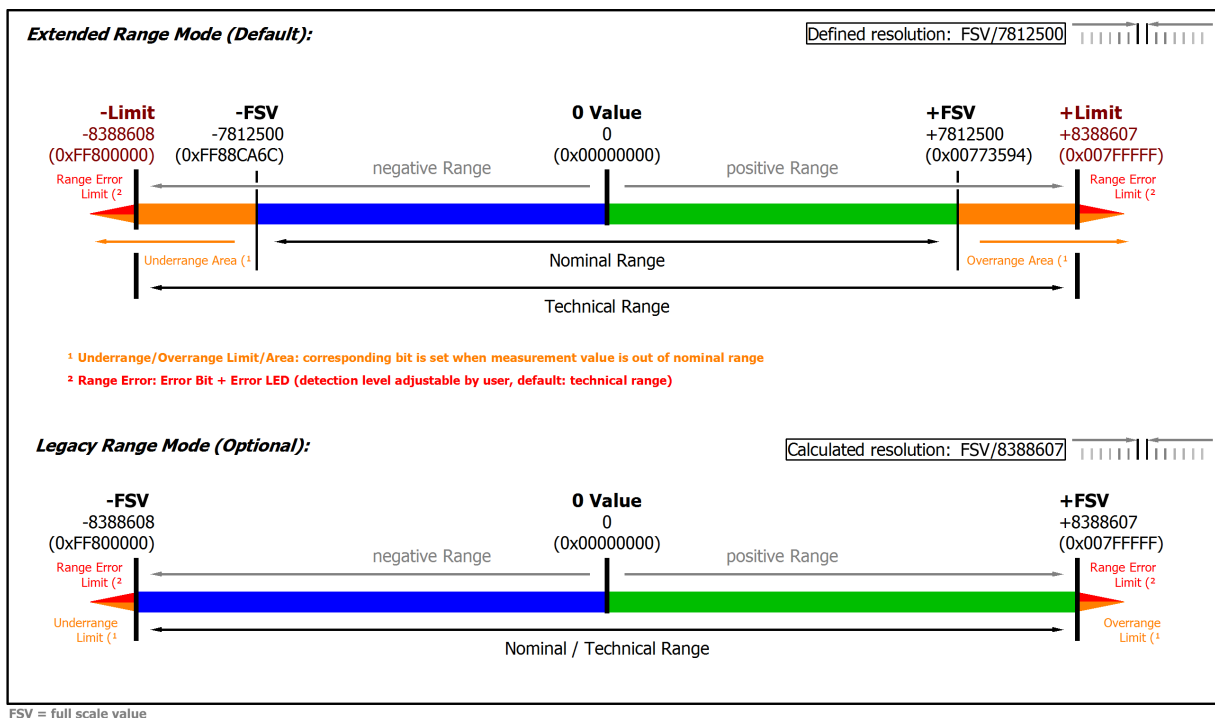
Fig. 49: Overview measurement ranges, Bipolar
