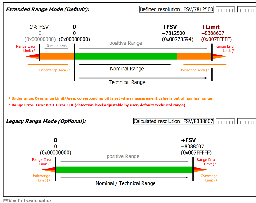
Fig. 69: Overview measurement ranges, Unipolar
