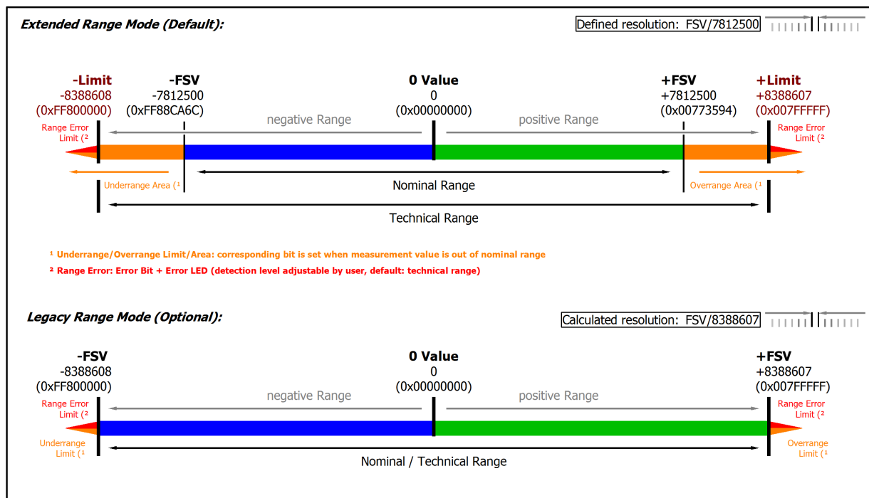
Fig. 90: Overview measurement ranges, Bipolar
