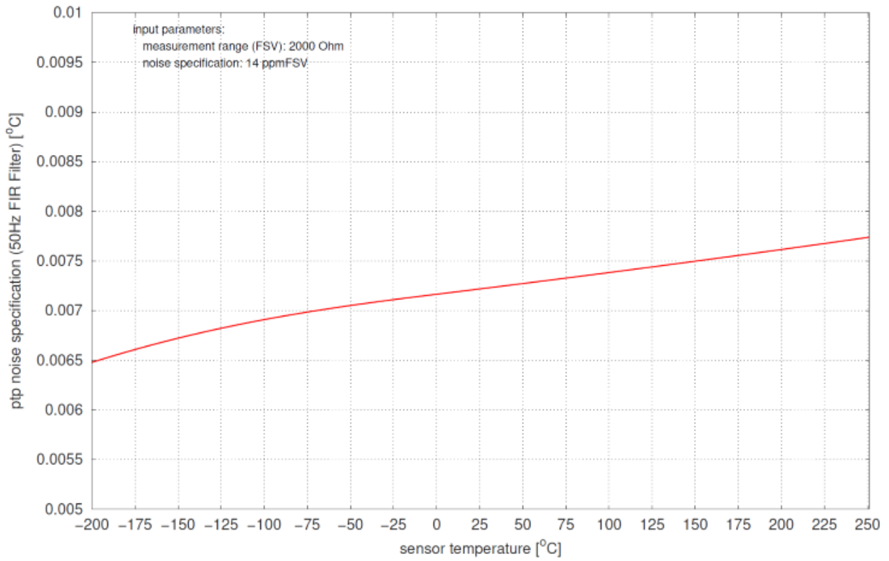
Fig. 85: Diagram noise E_{\text{Noise, PTP}} in dependence on sensor temperature
