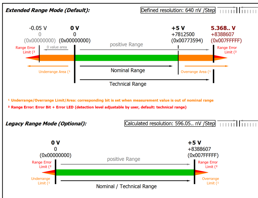
Fig. 119: Representation 0...5 V measurement range
