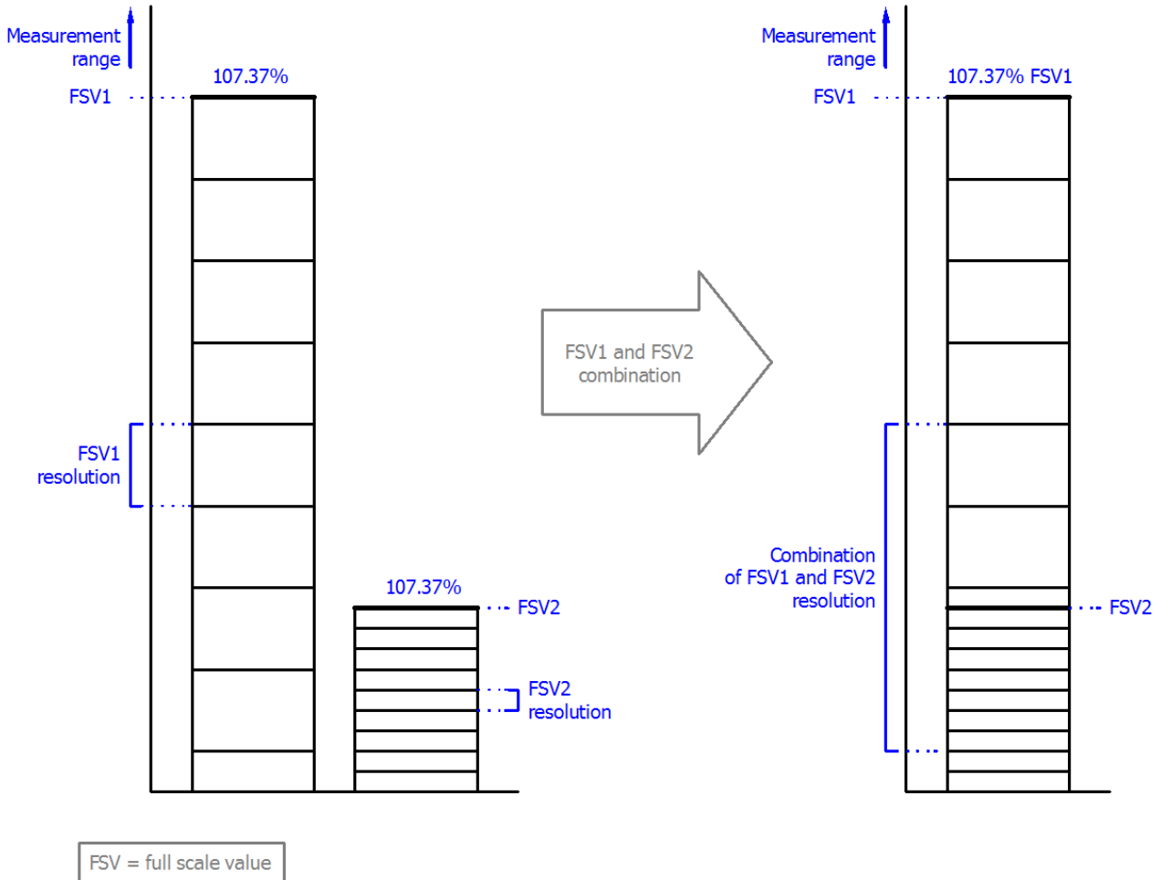
Fig. 208: Principle of combining two measuring channels with FSV1 and FSV2
