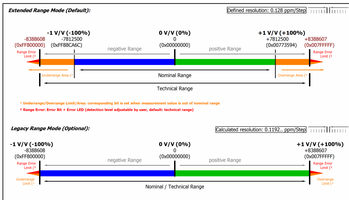
Fig. 141: Representation potentiometer measurement range
