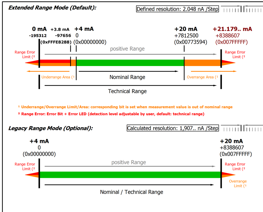
Fig. 130: Representation current measurement range 4...20 mA
