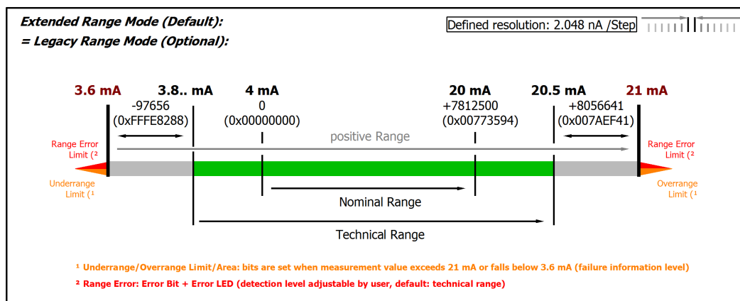
Fig. 172: Chart: current measuring range 3.6...21 mA (NAMUR)
