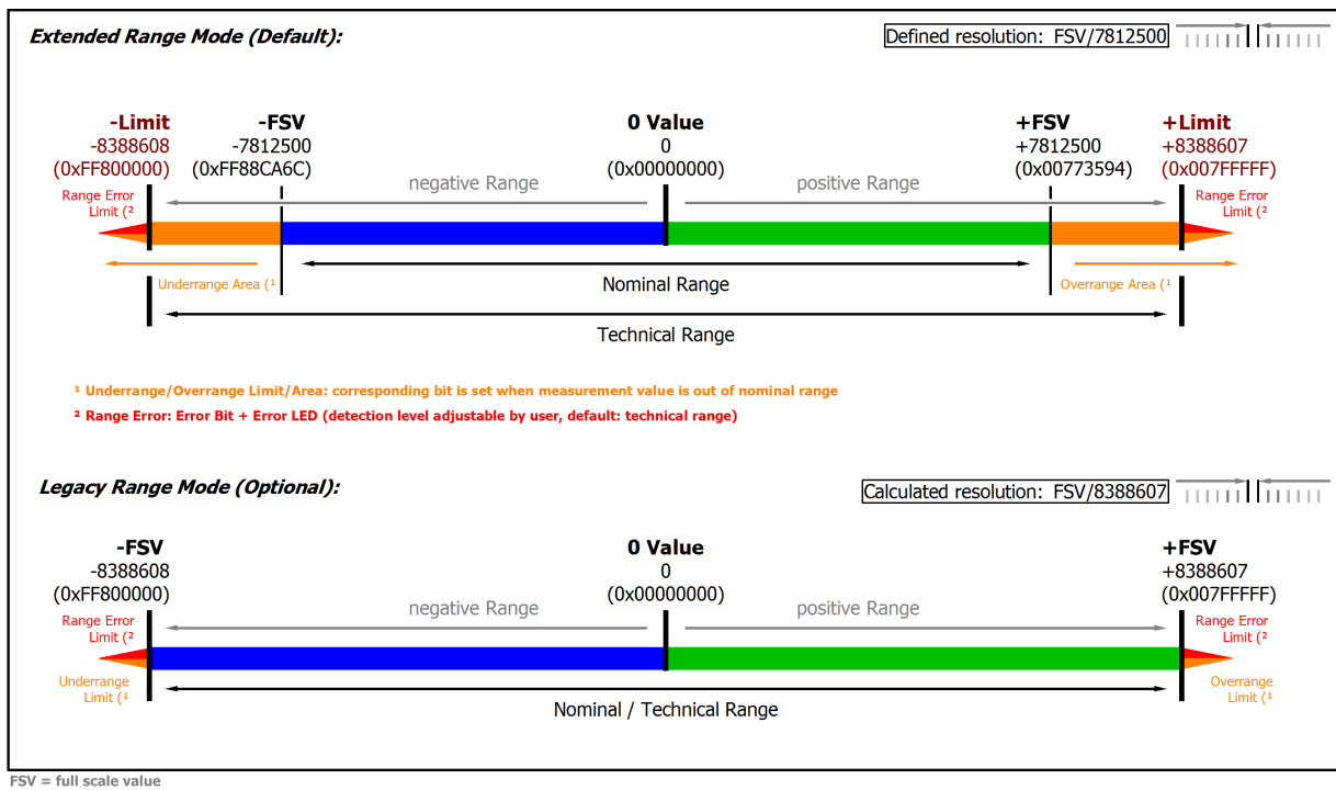
Fig. 79: Overview measurement ranges, Bipolar
