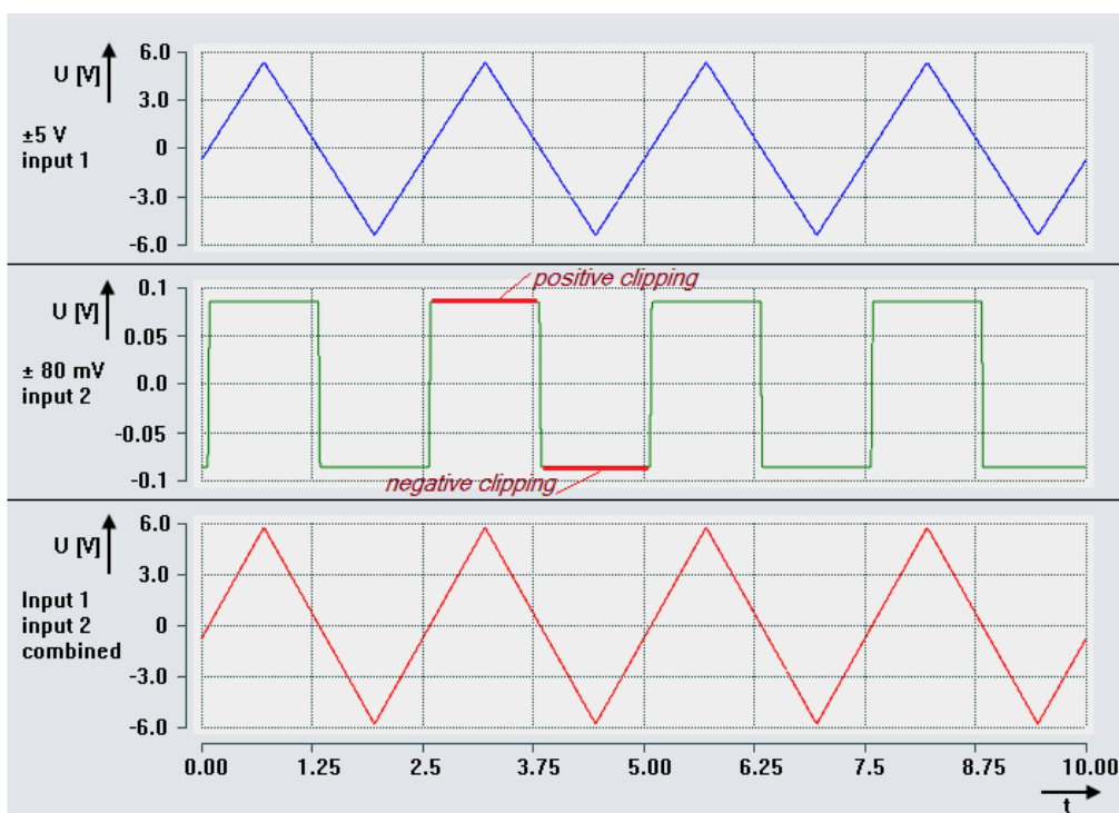
Fig. 210: Combination of two channels of the ELM3602-0002 with \pm 5 V and \pm 80 mV measuring range
