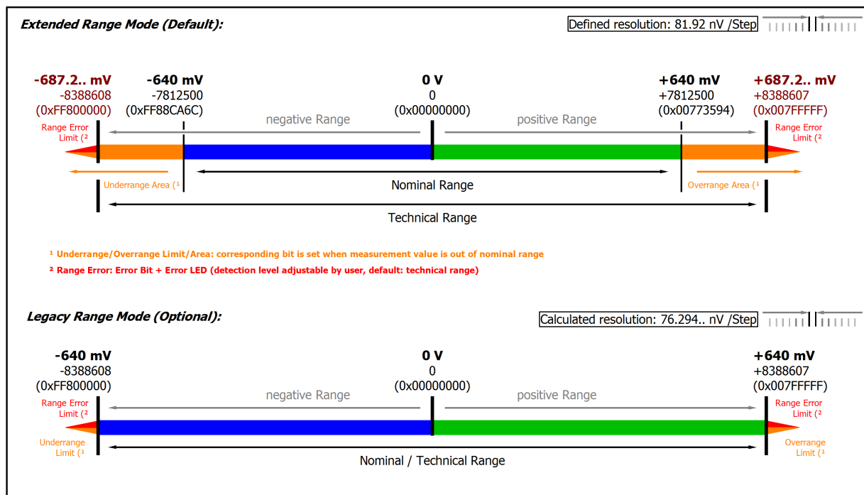
Fig. 15: Representation \pm 640 mV measurement range
