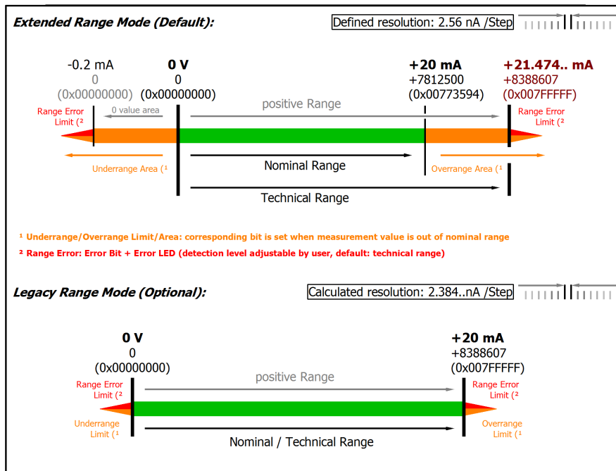
Fig. 45: Representation current measurement range 0...20 mA
