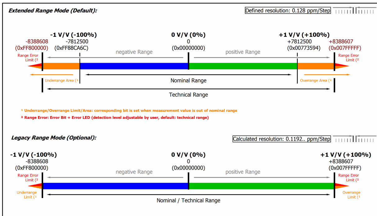
Fig. 86: Representation potentiometer measurement range
