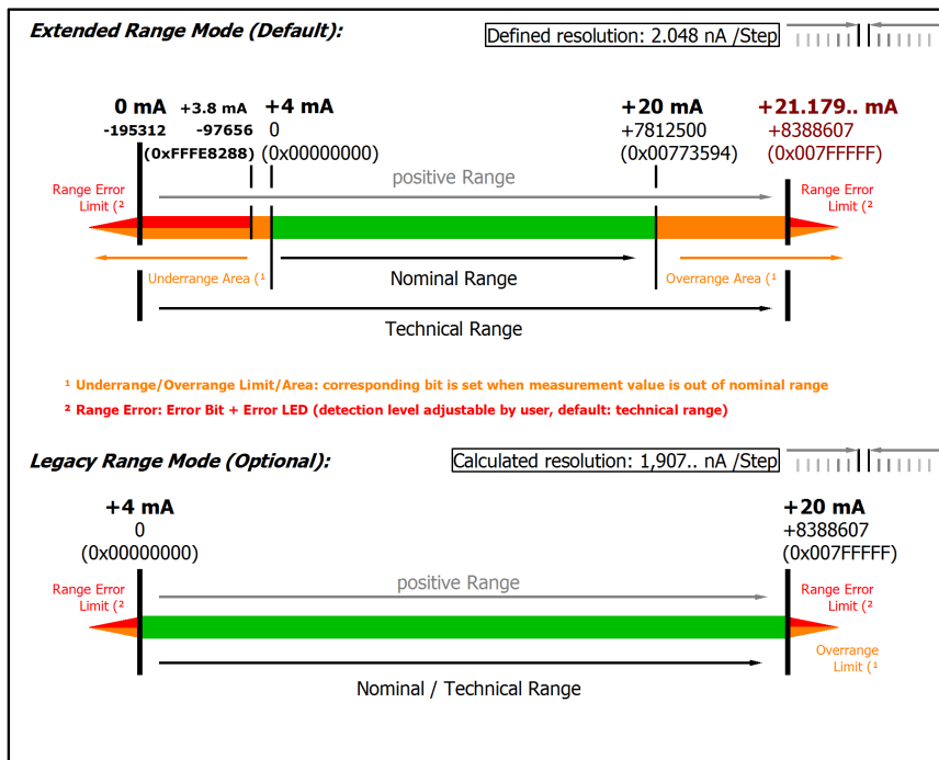
Fig. 65: Representation current measurement range 4...20 mA
