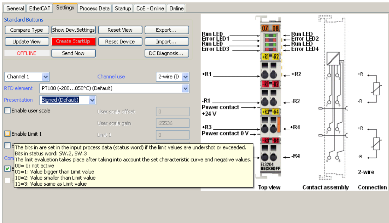
Fig. 223: Example of commissioning aid for a EL3204
