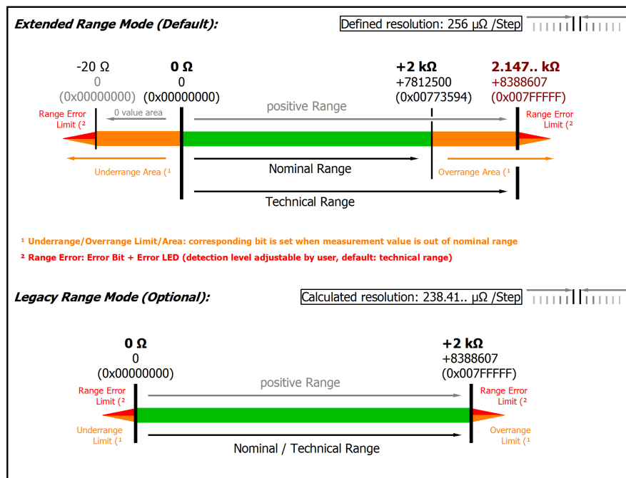
Fig. 133: Representation resistance measurement range 2 kΩ
