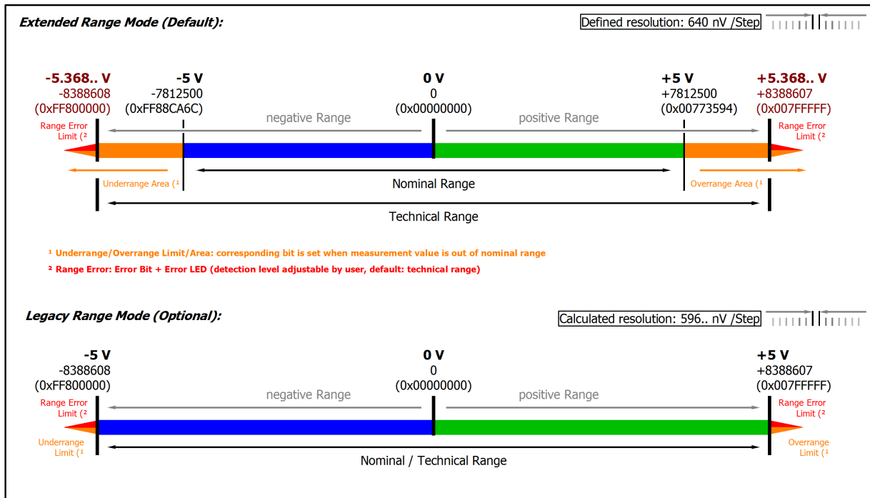
Fig. 98: Representation ±5 V measurement range
