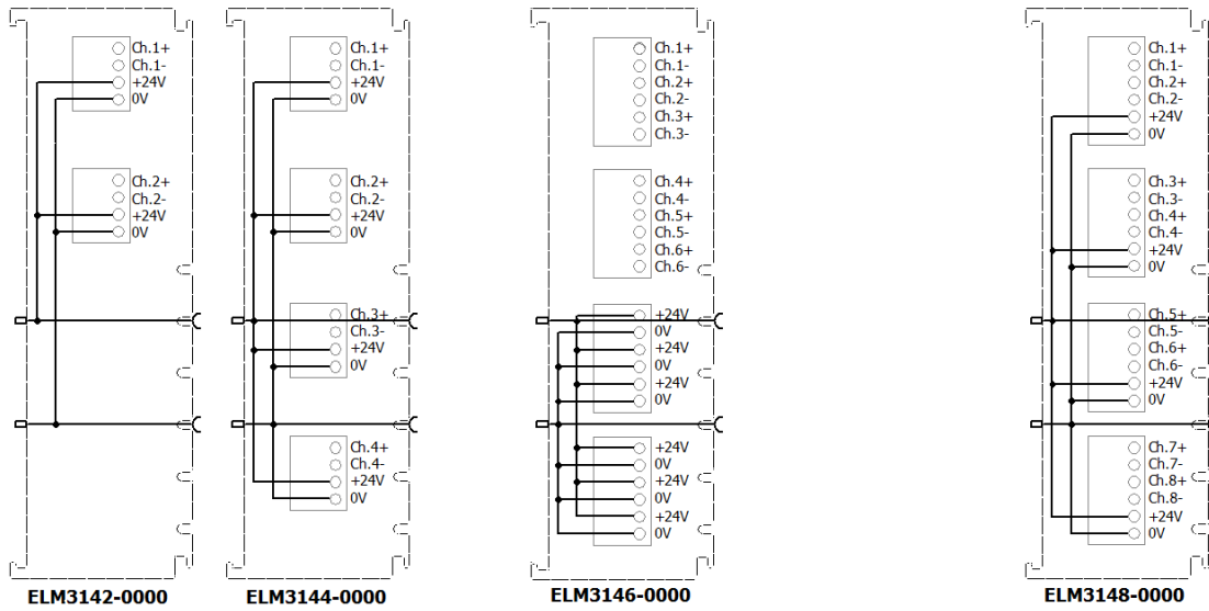
Fig. 365: Connections of the power contacts of the ELM314x
