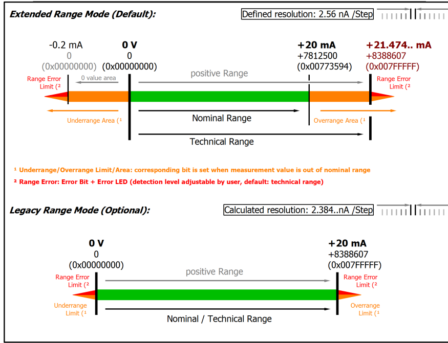
Fig. 129: Representation current measurement range 0...20 mA
