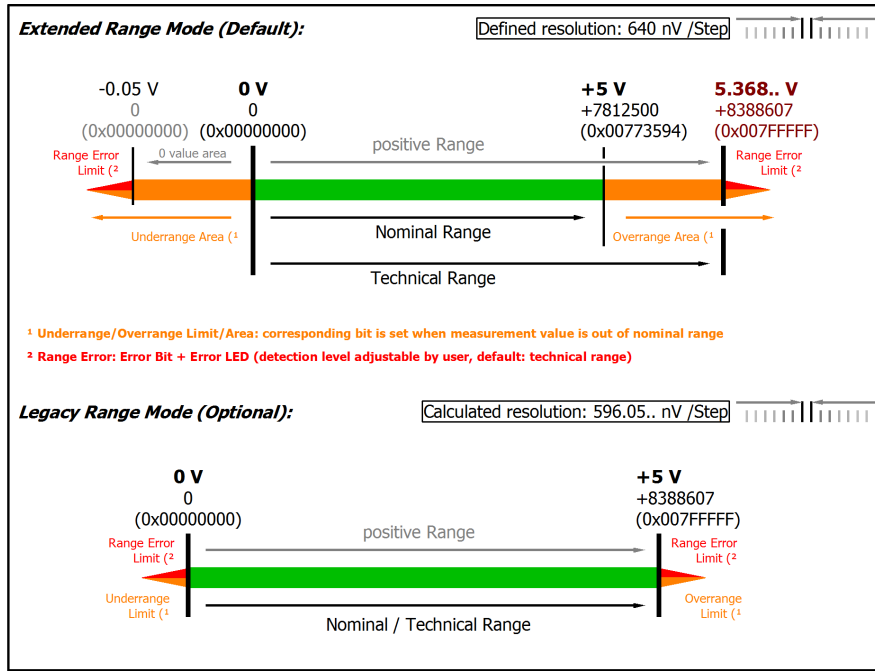
Fig. 57: Representation 0...5 V measurement range
