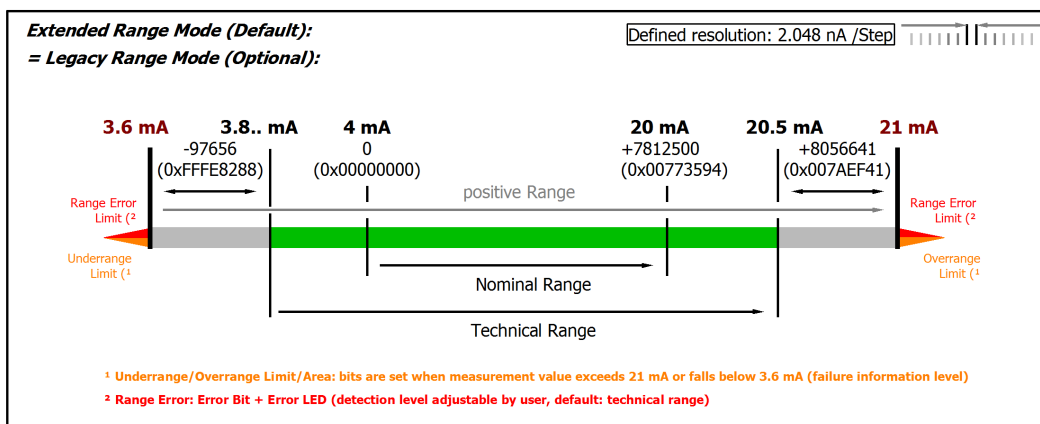
Fig. 47: Chart: current measuring range 3.6...21 mA (NAMUR)
