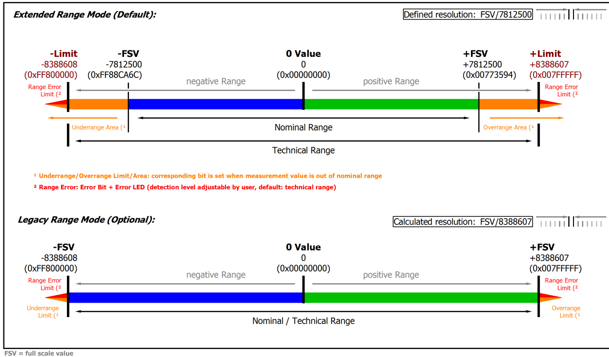
Fig. 22: Overview measurement ranges, Bipolar
