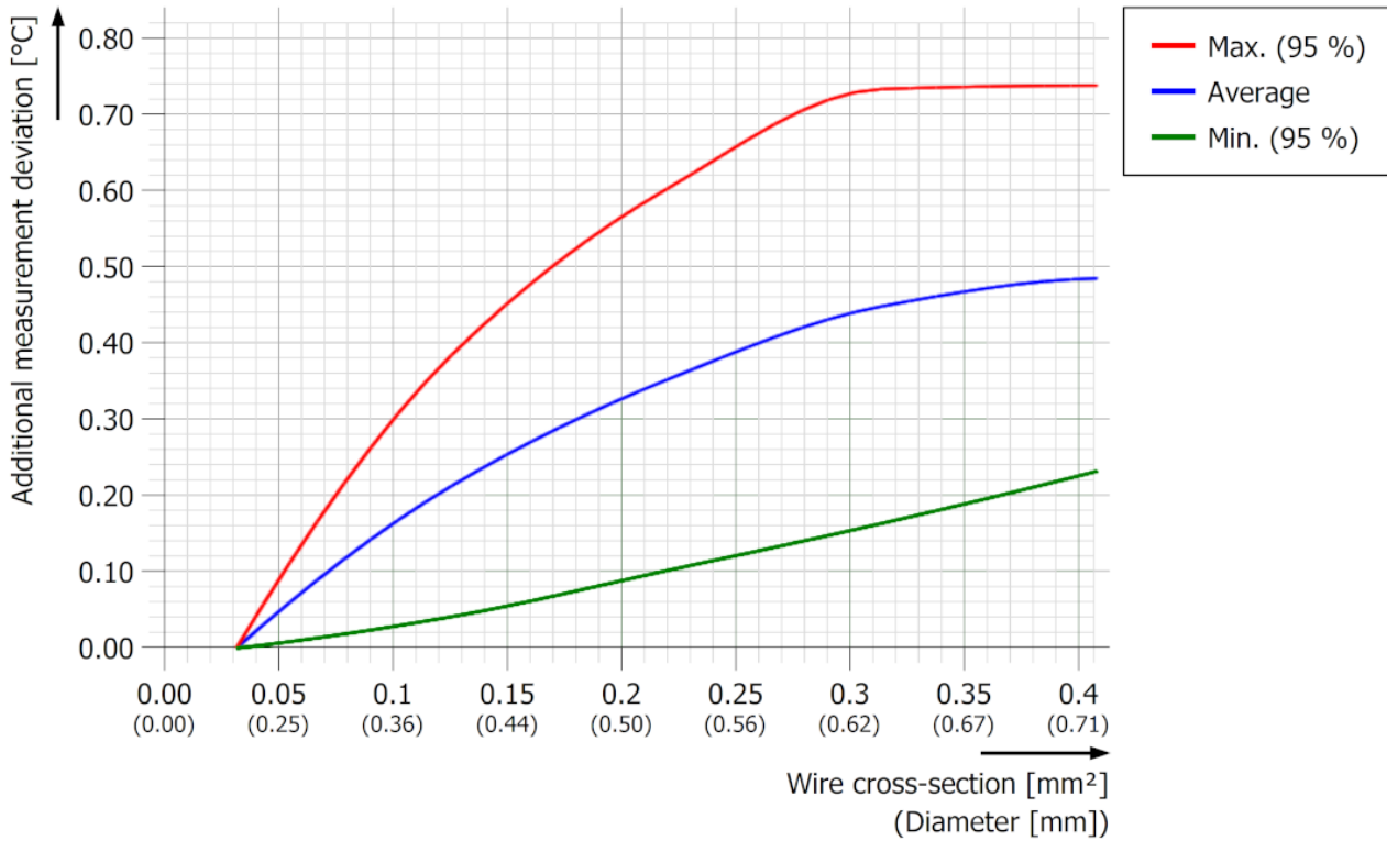
Fig. 152: Additional deviation over TC wire cross-section/ diameter of ELM370x-0000 with push-in plug
