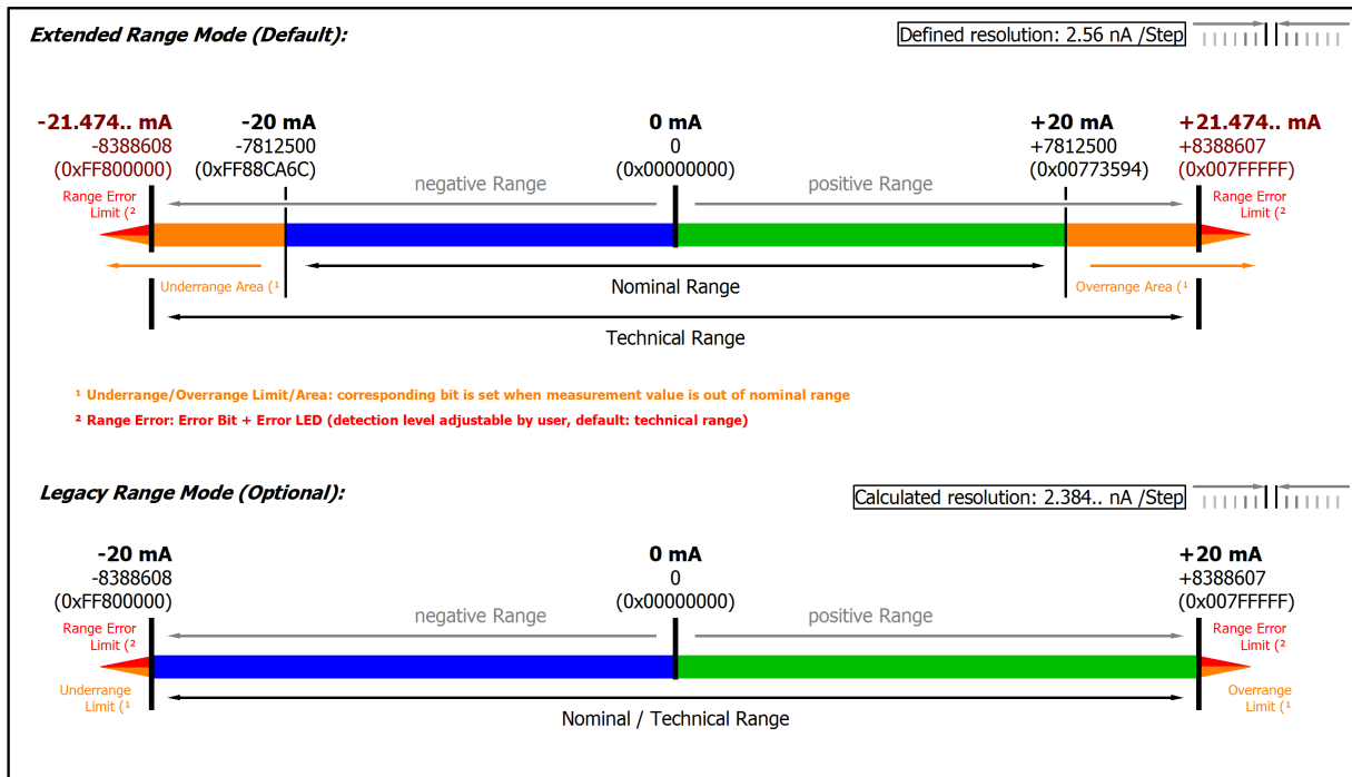
Fig. 24: Representation current measurement range ±20 mA
