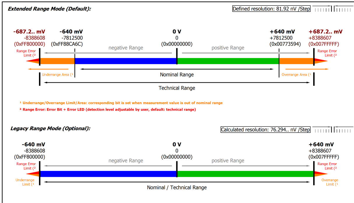
Fig. 163: Representation ±640 mV measurement range
