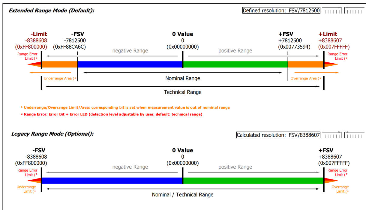
Fig. 154: Overview measurement ranges, Bipolar
