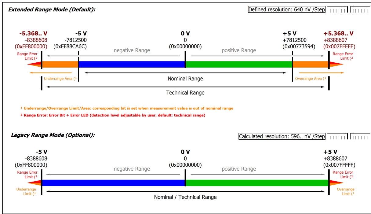
Fig. 159: Representation ±5 V measurement range
