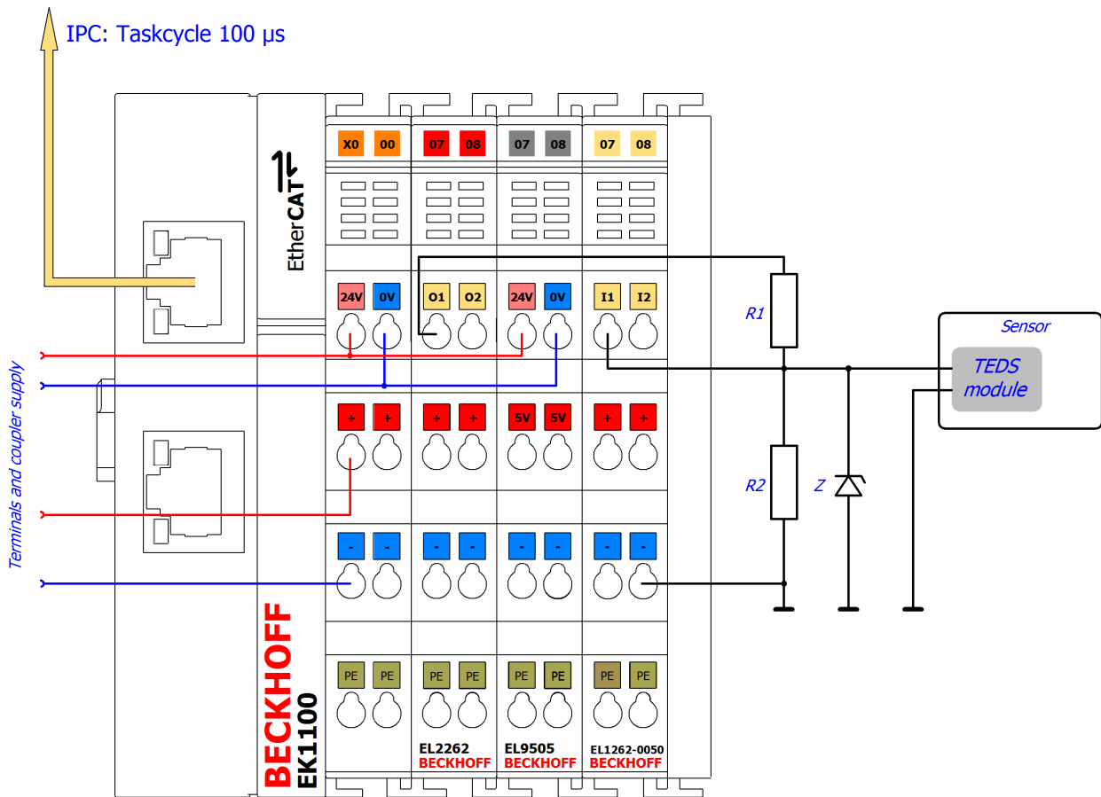
Fig. 212: Wiring for sample program 3
