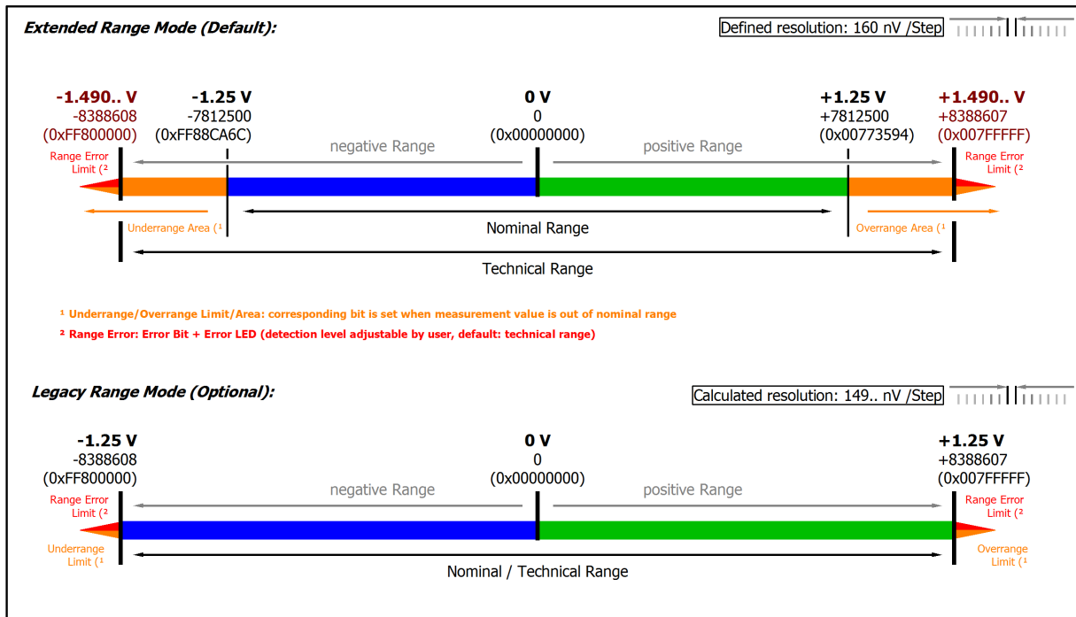
Fig. 61: Representation ±1.25 V measurement range
