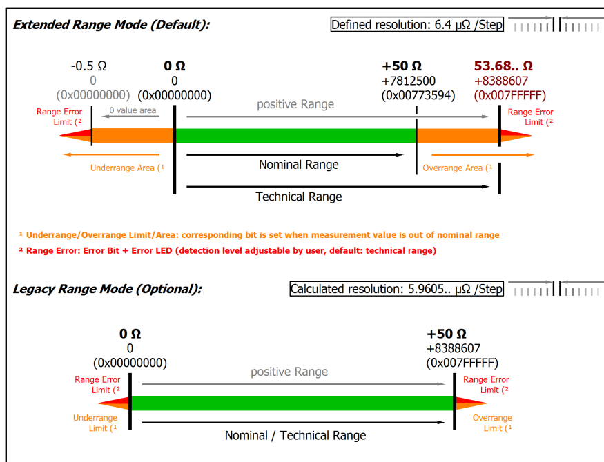
Fig. 136: Representation resistance measurement range 50 Ω
