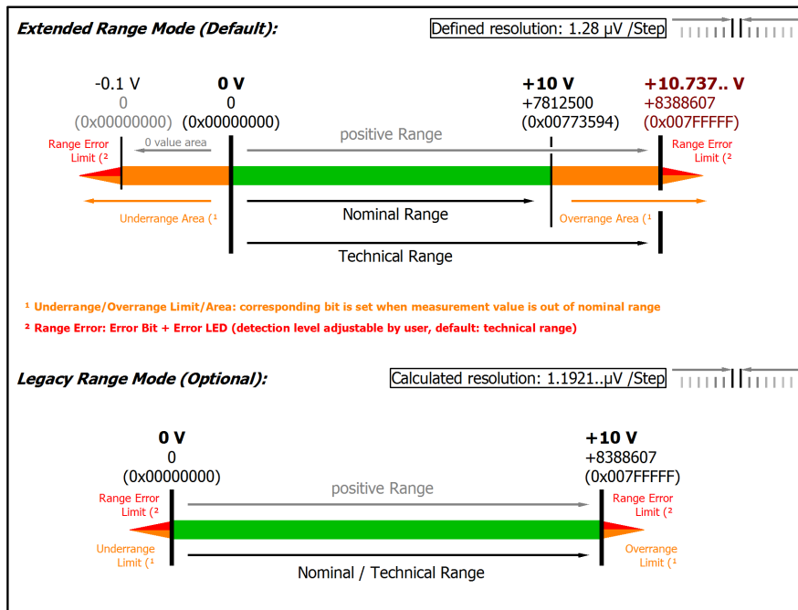
Fig. 186: Representation 0...10 V measurement range
