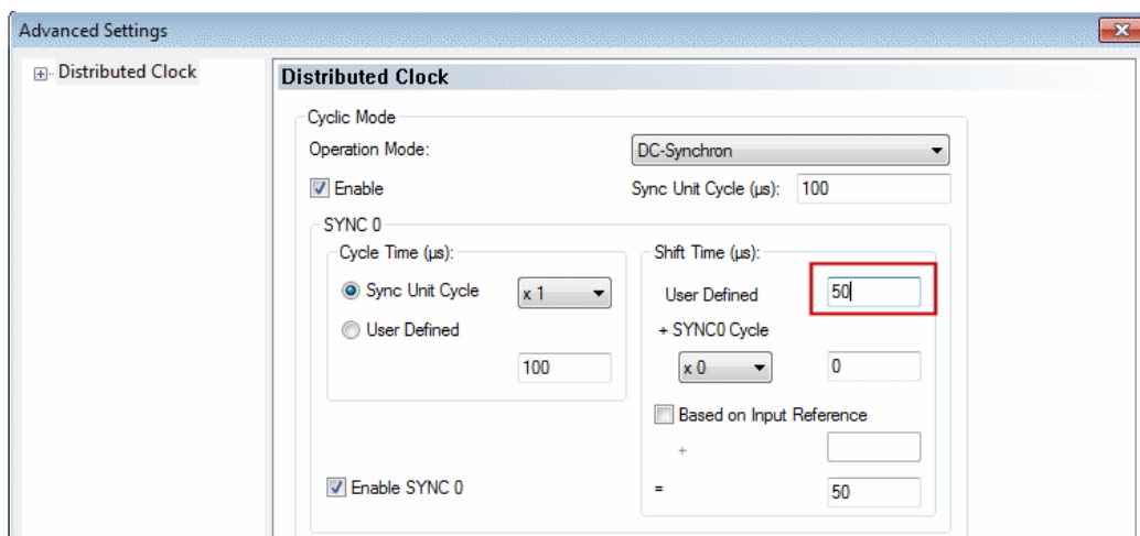
Fig. 204: Setting the DC shift time for terminal 2
