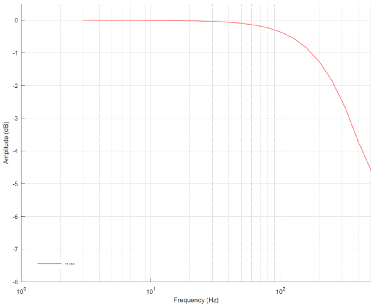
Fig. 52: Frequency response of measuring range \pm 10\text{ V} , f_{\text{sampling}} = 1\text{ kHz} , integrated filters 1/2 deactivated
