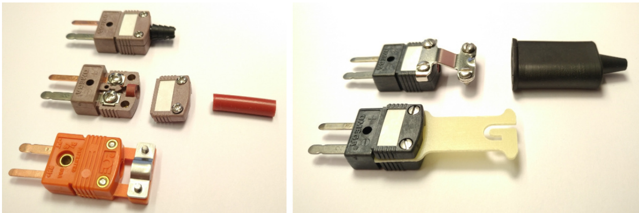
Fig. 338: Left: recommended strain reliefs/sealing ring/kink protection, without mounting height; right: non-permissible strain reliefs, with mounting height
