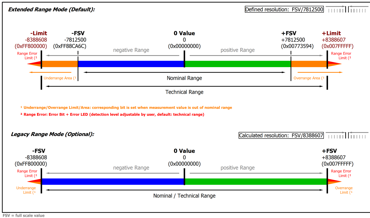
Fig. 29: Overview measurement ranges, Bipolar
