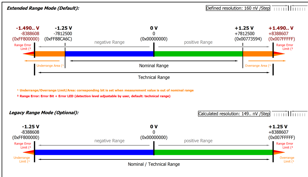
Fig. 14: Representation \pm 1.25 V measurement range
