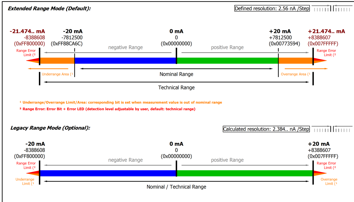
Fig. 44: Representation current measurement range ±20 mA
