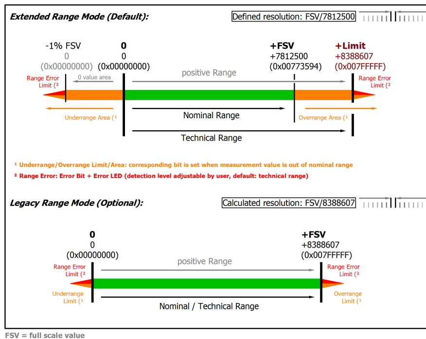
Fig. 80: Overview measurement ranges, Unipolar
