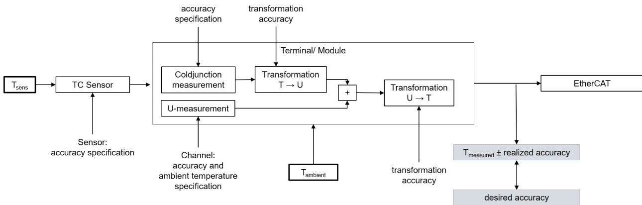
Fig. 75: Concatenation of the uncertainties in temperature measurement with thermocouples
