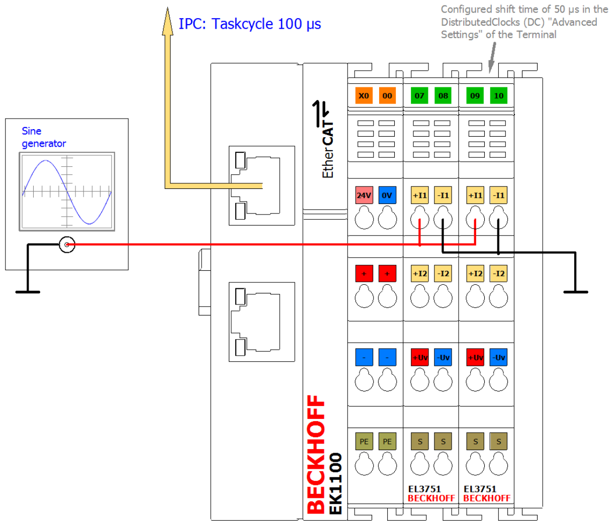
Fig. 203: Configuration and setup for sample program 6: Doubling of the sample rate with 2 x EL3751
