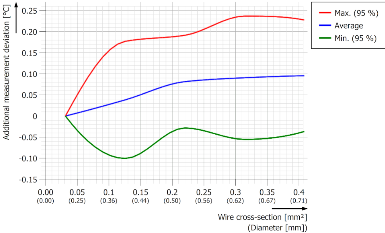
Fig. 77: Additional deviation over TC wire cross-section/ diameter of ELM334x-0000 with push-in plug
