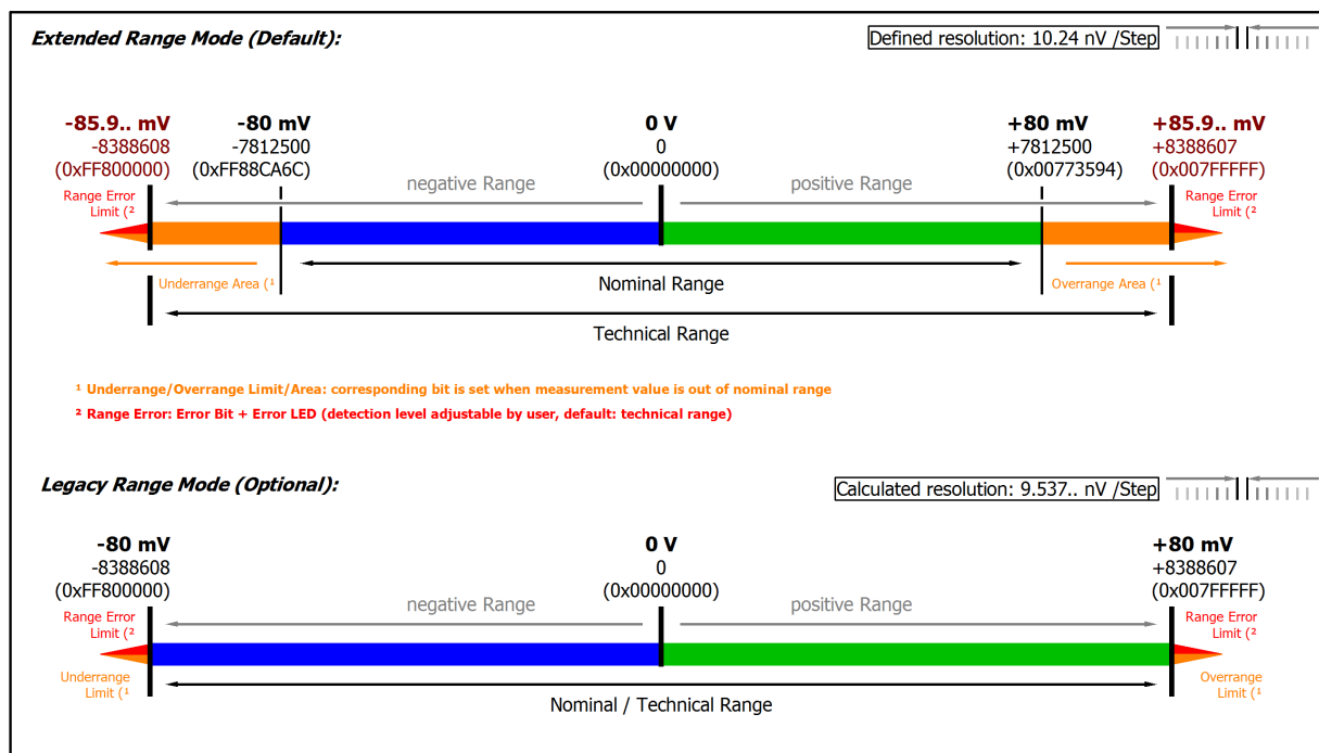
Fig. 82: Representation \pm 80 mV measurement range
