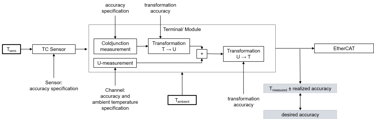
Fig. 191: Concatenation of the uncertainties in temperature measurement with thermocouples
