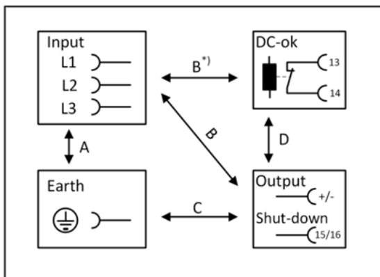
Fig. 19: Dielectric strength
