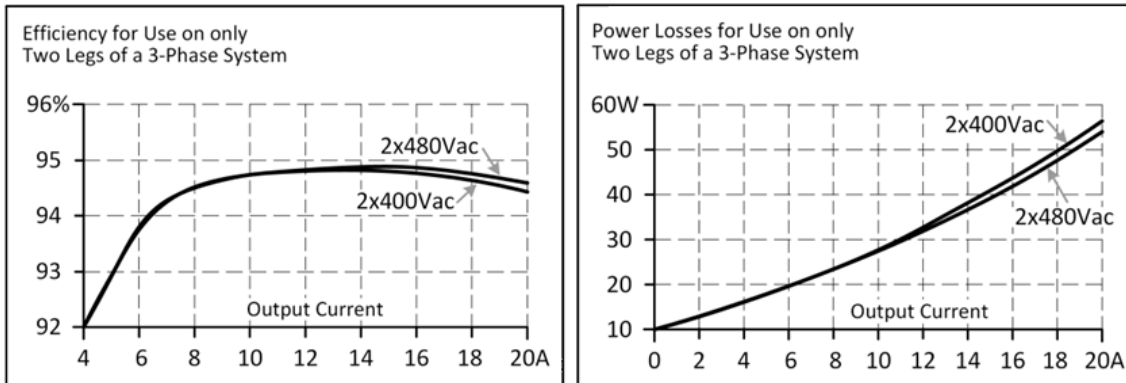
Fig. 14: Efficiency over output current at 48 V; losses over output current at 48 V
