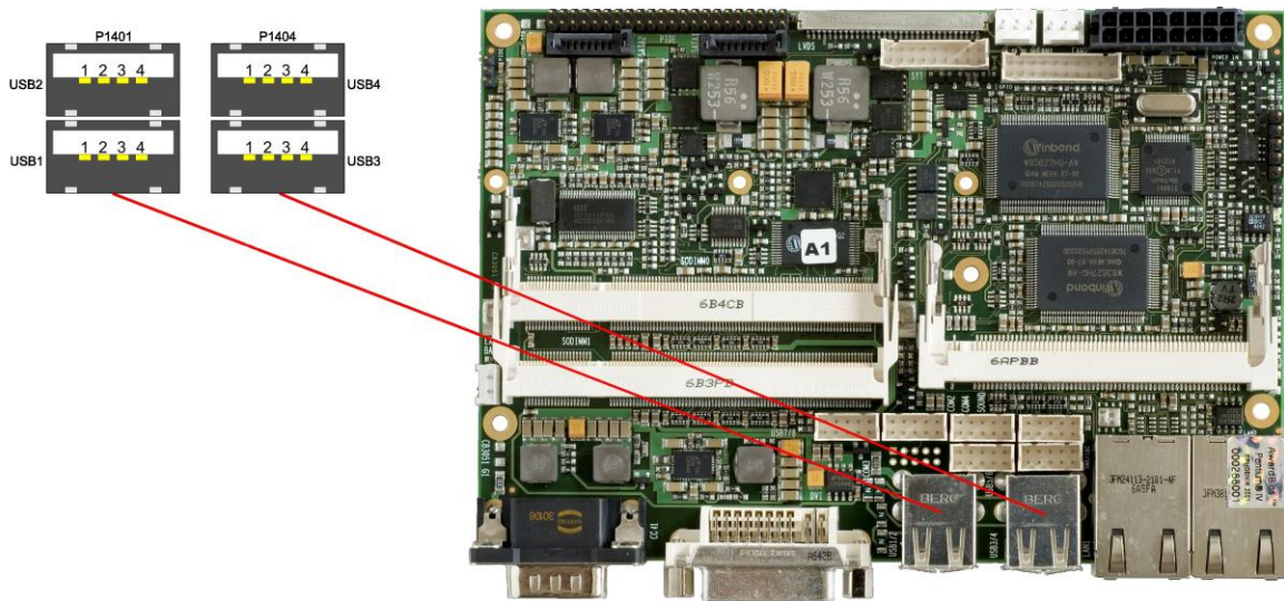
Pinout USB connector for channel X:
