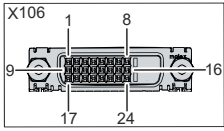
Fig. 8: DVI-Extended input pin numbering
