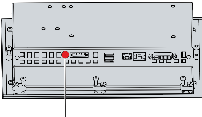
Fig. 13: Ground connection Functional earthing
