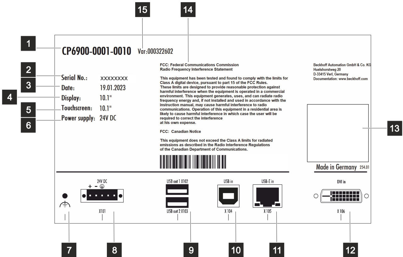
Fig. 9: Name plate
