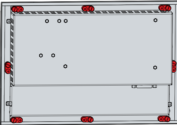
Fig. 10: Delivery state clamping lever
