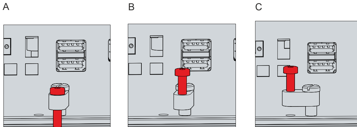
Fig. 16: Removal from the control cabinet
