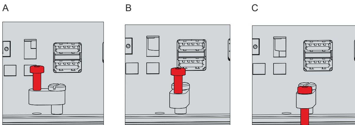
Fig. 12: Control cabinet installation
