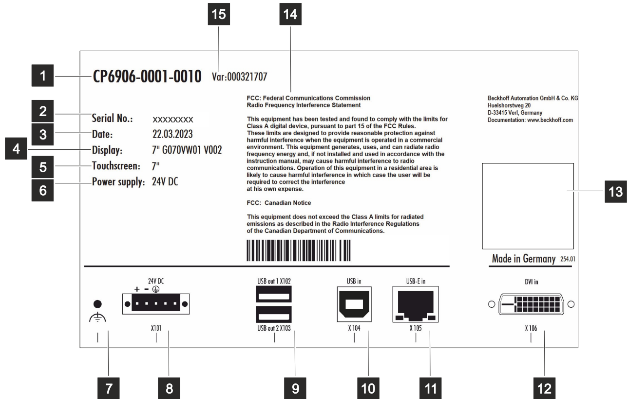
Fig. 9: Name plate
