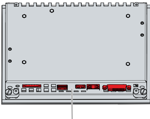
Fig. 3: Connection section
