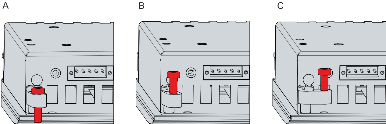
Fig. 16: Removal from the control cabinet
