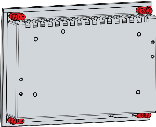
Fig. 10: Delivery state clamping lever
