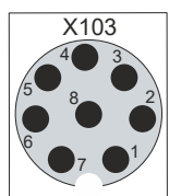
Fig. 5: CP79xx_USB-E 2.0 input pin numbering
