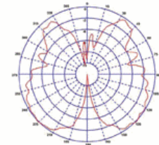
2400 MHz Elevation
