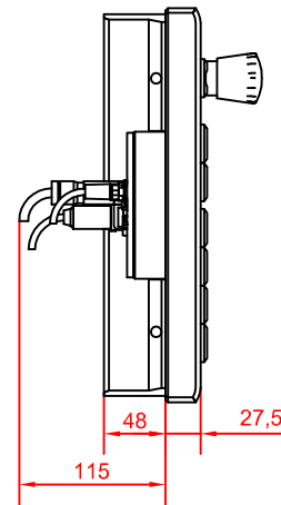
left view
