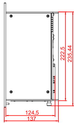
left view
