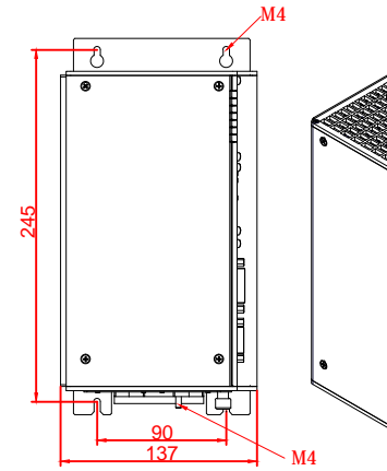
left view
